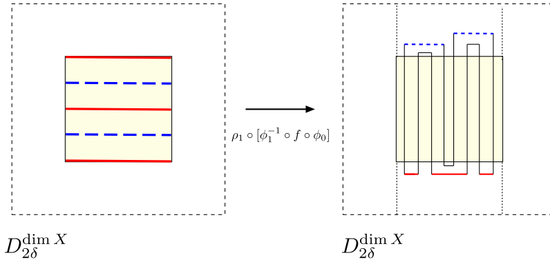
FIGURE 2. Illustration of the isotopy creating a pseudo-horseshoe.
