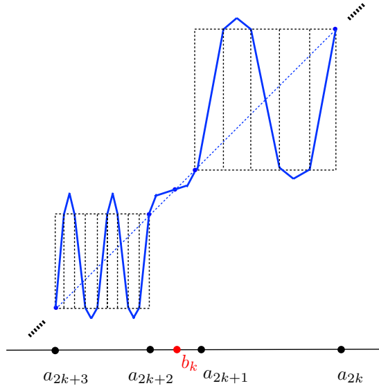
FIGURE 4. Local construction of an attractor between two consecutive pseudo-horseshoes.
