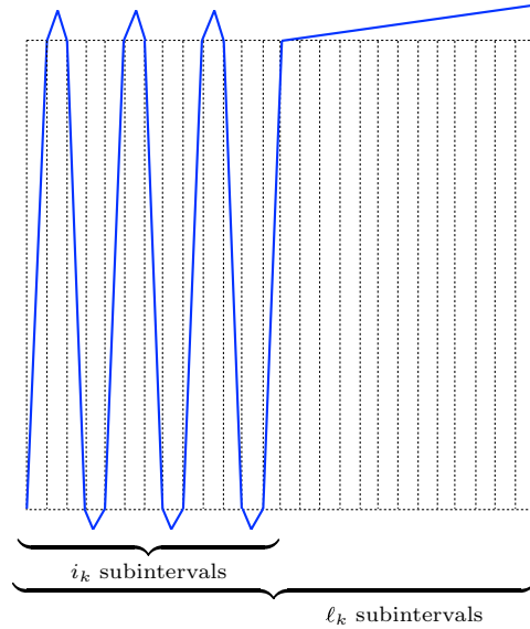
FIGURE 3. Selection procedure of piecewise linear components of f_\beta .
