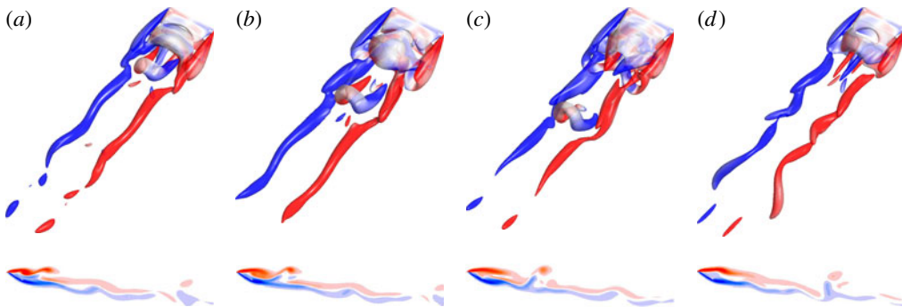
FIGURE 11. (Colour online) Top row: top-down angled view of the isosurface for Q=10 coloured by streamwise vorticity behind an AR=2 trapezoidal plate at \Lambda = 10^\circ, \alpha = 30^\circ and Re = 300 . Bottom row: corresponding spanwise vorticity plots in the centre plane showing the leading-edge shedding that is associated with the observed lift coefficient variation. The surfaces correspond to the times marked in figure 10(c): (a) t_1 ; (b) t_2 ; (c) t_3 ; (d) t_4 .
