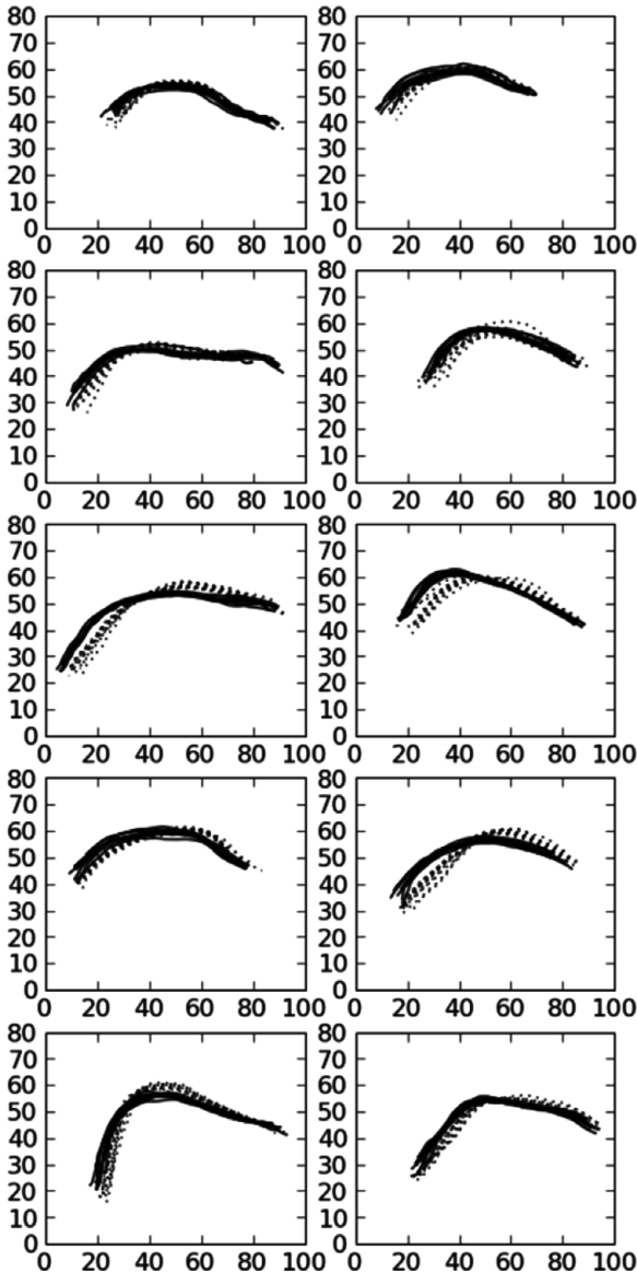
Figure 2 Tongue contours for ten repetitions of s_a (solid curves) and ten repetitions of s_i (dotted curves) in all adult speakers. Adults 1–5 are on the left, and Adults 6–10 are on the right.
