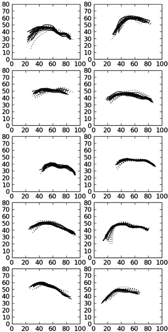
Figure 3 Tongue contours for ten repetitions of s_a (solid curves) and ten repetitions of s_i (dotted curves) in all child speakers. Children 1–5 are on the left, and Children 6–10 are on the right.
