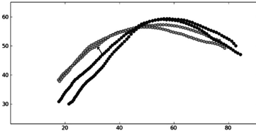
Figure 1 Two s_a curves (light circles) and two s_i curves (black circles), produced by the same speaker. An arrow represents the nearest neighbour distance from a point on a s_i curve to one of the s_a curves. The scale is in millimetres.
