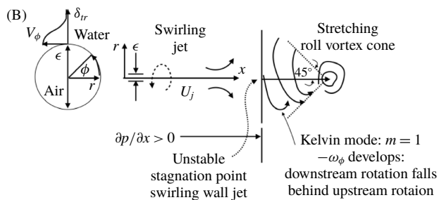
FIGURE 7. Vortex breaking, jetting, reconnection and stretching along 45^\circ to flow direction just prior to terminal bursting (a,b), and mechanism of formation of roll vortex at vortex tip (c). (a,b) These sequences take place after the slant \beta of the main root vortex reaches 45^\circ ; repeated jetting and spiralling at vortex tip are shown, and formation of spiralling cones and stretching along 45^\circ are shown. (c) Insets 1 and 2 in (A) show examples of ‘vortex rods’ which are swirling jets as in (a2); (B) schematic of the mechanism of the formation of the roll vortex cones at the tip of the swirling jets shown in (a,b).
