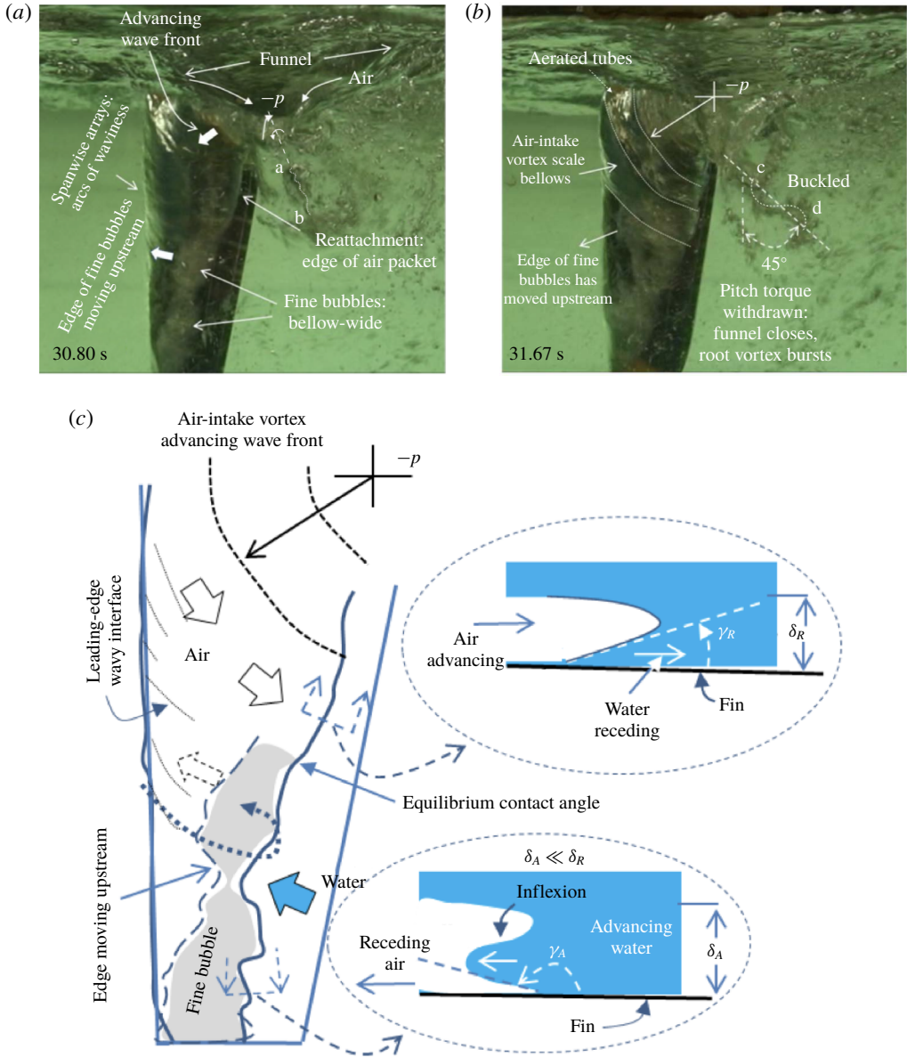
FIGURE 10. Formation of fine bubbles on the foil surface: time sequence of air jacket and regions of clouds of fine bubbles over the suction side of the fin (a,b); schematic of surface tension mechanism of the formation of fine bubbles (c). Two elliptical insets in (c) show cross-sections of areas where the foil surface and the air and water interfaces meet. In (a), the markings ‘a’ and ‘b’ draw attention to an extremely thin aerated vortex with small amplitude waves, aligned with the centre of the funnel; when stretched to the maximum extent due to the 45° slope, this vortex buckles to a sinusoid marked (c,d) in (b).
