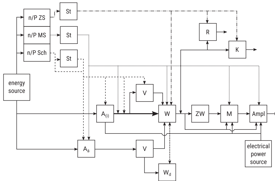
Figure 6. General musical instrument system (adapted from Heyde 1975: 62). For abbreviations, see Table 1. Additionally, Heyde annotates certain elements with subscripts: A_i stands for internal activator ( Anreger für innere ), A_a for external activator ( Anreger für äußere ) and W_d for double transducer ( Doppelwandler ).
