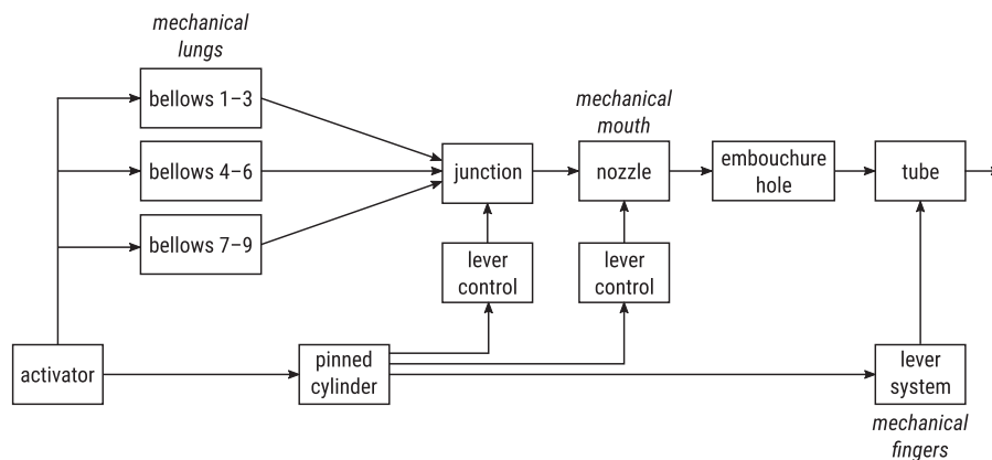
Figure 9. Network for Vaucanson’s flute-playing android (adapted from Heyde 1975: 26).
