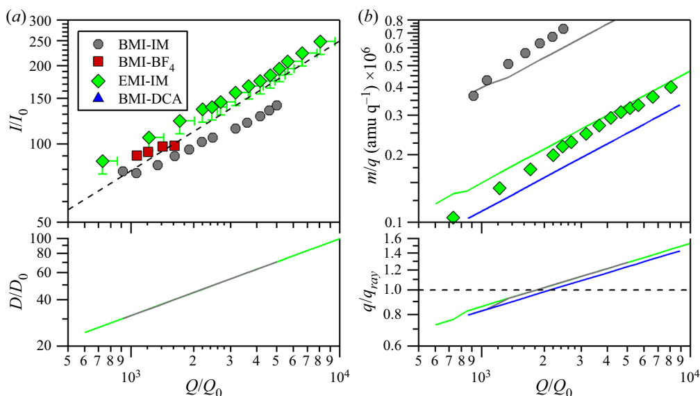
Figure 8. Comparison of the emitter output per dimensionless flow rate for the electro sprayed ILs BMI-IM, BMI-BF 4 , EMI-IM and BMI-DCA using the dimensionless scaling laws of Gañán-Calvo et al. (2018); (a – top) dimensionless current output with the dashed line representing the theoretical prediction; (a – bottom) theoretical prediction of the dimensionless mean droplet diameter. The results overlap for each IL, thus only two are illustrated; (b – top) theoretical and experimental m/q values of the mean droplet shown for three ILs; (b – bottom) theoretical ratio of droplet mean charge to Rayleigh charge limit. The initial emitted mean droplets are expected to be super Rayleigh above Q/Q_0 = 2147 .
