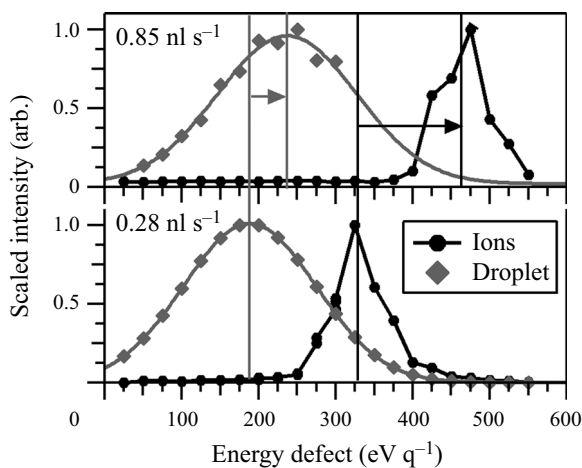
Figure 6. Integrated ion peaks and droplet distributions of EMI-IM charged particles that have been scaled to allow for comparison of the relative FWHM and centroid values at two flow rates. The vertical lines mark the centroids of a Gaussian fit to each data set and the arrows indicate the direction of shift with increasing flow rate.
