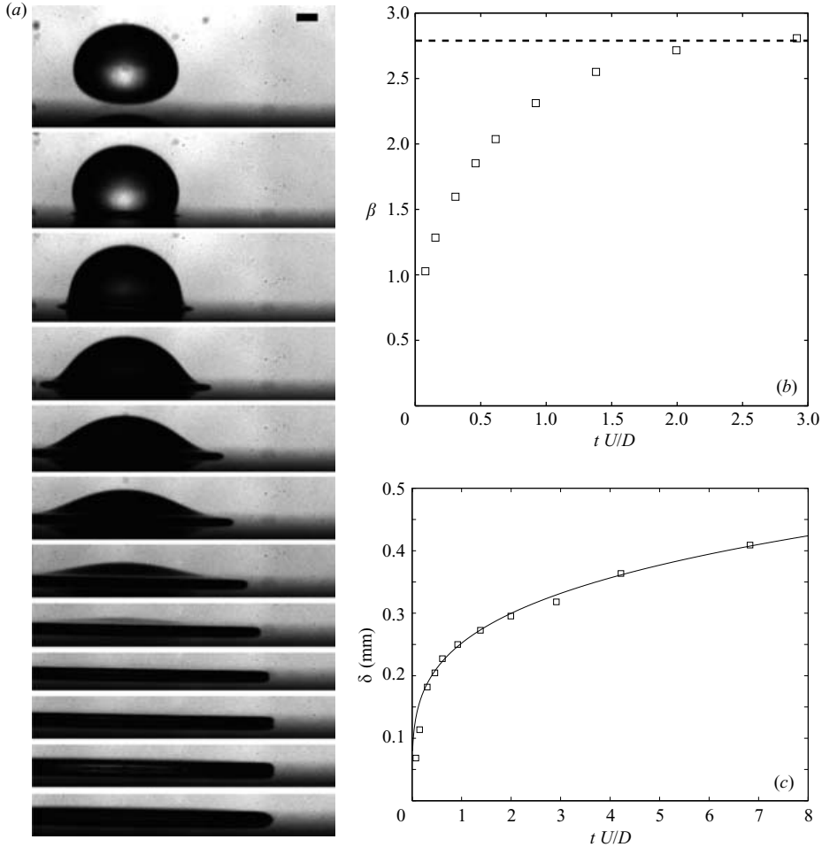
FIGURE 6. The impact of a viscous drop onto a dry glass plate, Re_d = 460 and We_d = 5720 . (a) The evolution of the impact lamella travelling along the plate. The times shown are -50, 50, 100, 200, 300, 400, 600, 900, 1300, 1900, 2750 and 4450 \mu\text{s} after first contact. The scale bar is 1 mm long. (b) The spread-factor \beta vs. the normalized time. (c) The thickness of the lamella travelling along the plate. The solid curve shows the power law \delta \sim (tU/D)^{0.25} .
