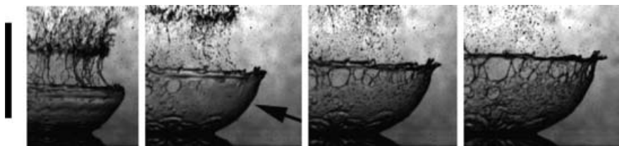
FIGURE 8. The appearance of Marangoni patches in the crown. The arrow points to a region of the crown which is free of pock-marks. Subsequent frames show the appearance of numerous patches, which we interpret as the impact of ethanol droplets, which are projected downwards from the broken ethanol sheet. The frames are taken at 1.1, 1.5, 1.7 and 1.9 ms from first contact. The scale bar is 10 mm long.
