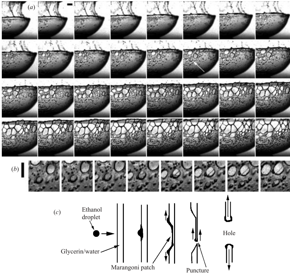
FIGURE 3. The formation of holes in the crown. (a) The arrow in frame 14 points to a Marangoni patch, where the thin film is in the process of puncturing. The frames are spaced by 20 \mu\text{s} , going from left to right and then top to bottom, spanning a total of 620 \mu\text{s} . (b) Close-up of the rupture of the patch identified in (a). One can also see another patch rupture directly below it. The scale bars are 1 \text{ mm} . (c) Sketch of the three stages in the formation and growth of holes.
