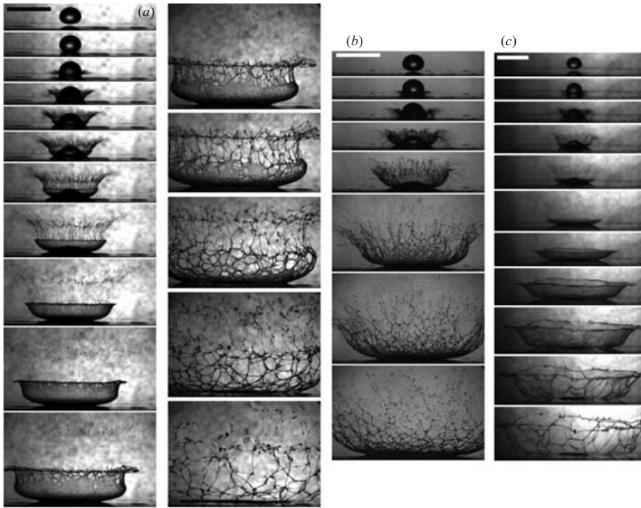
FIGURE 7. The impact of different viscosity drops. (a) Drop is 94 % glycerin, Re_d = 250 and We_d = 5780 . Times shown are -50, 0, 50, 100, 150, 200, 300, 450, 650, 900, 1200, 1550, 2000, 2550, 3300 and 4750 \mu\text{s} after first contact. (b) The impact of a lower viscosity drop (83 % glycerin), Re_d = 1100 and We_d = 5600 . Times shown are -20, 40, 100, 400, 900, 1280 and 1840 \mu\text{s} after first contact. (c) Higher viscosity drop, (99 % glycerin), Re_d = 95 and We_d = 5600 . Times shown are -50, 50, 150, 250, 350, 600, 1200, 2000, 2700, 3100 and 4000 \mu\text{s} . All bars 10 mm.
