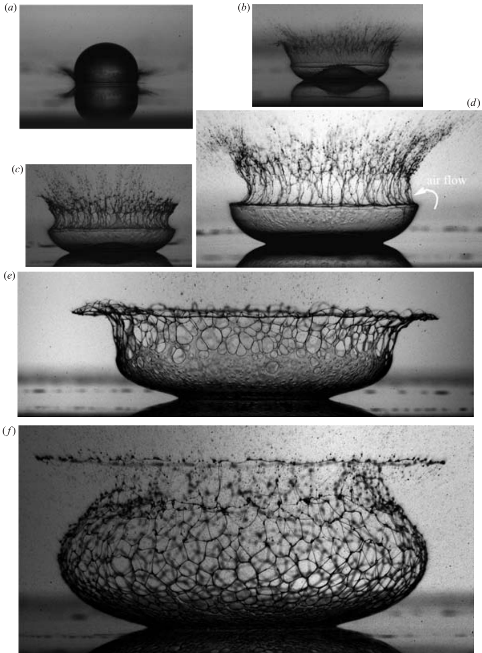
FIGURE 4. Still images taken during the impact of different drops, under similar conditions as in figure 1. (a) Initial splashing. (b) Continuous ethanol sheet. Note the bubble under the drop. (c) Breakup of ethanol sheet. (d) Ethanol sheet breaks up into filaments. (e) Formation of holes. Notice the thicker edge. (f) Network of liquid filaments. Images are not to the same scale.
