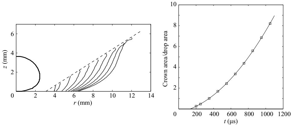
FIGURE 5. (a) The crown shapes are shown at 200, 250 and thereafter at intervals of 100\ \mu\text{s} after first contact of the drop. The crown height vs. its radius r is approximated by z = 0.62(r - R) , where R is the drop radius. The drop shape at first contact is also shown. (b) The crown area vs. time. The area is normalized by the original drop area.
