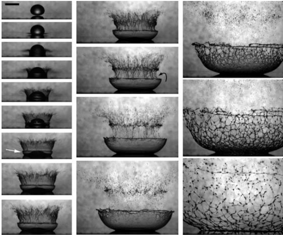
FIGURE 1. The impact of a viscous drop onto a 35\ \mu\text{m} film of ethanol. Drop is 89 % glycerin, giving Re_d = 460 and We_d = 5720 . Times shown are 0, 50, 100, 150, 200, 250, 350, 450, 550, 650, 800, 1050, 1400, 2000, 2800 and 4600\ \mu\text{s} after first contact. The scale bar is 5 mm long. See also the movie available with the online version of the paper.
