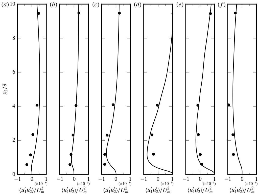
FIGURE 9. Profile of Reynolds stress (u'_1 u'_2)_{rms} , for several phase angles. Full line: DNS; circles: experimental data from Jensen et al. (1989) Test 6 with Re = 990 . (a) 5°; (b) 40°; (c) 73°; (d) 107°; (e) 140°; (f) 175°. Note that first value is taken at x_2/\delta = 9 \times 10^{-3} .
