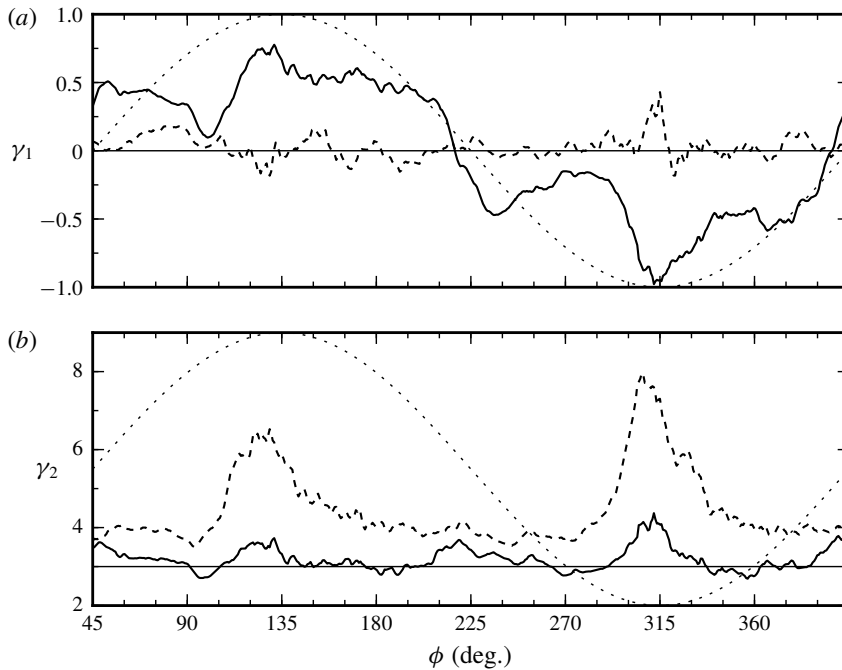
FIGURE 16. Statistics of wall vorticity fluctuations \Omega'/\Omega_{rms} . (a) Skewness; (b) kurtosis; Dashed line \Omega_1 ; full line \Omega_3 ; — \gamma_1 and \gamma_2 for normal distribution; \cdots as in figure 5.
