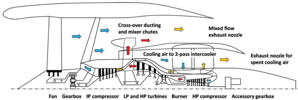
Figure 2. (Colour online) Schematic diagram of a reverse-flow-core intercooled turbofan aeroengine arrangement.
