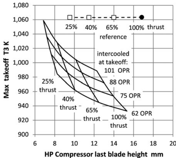
Figure 21. Max take-off T 3 for the conventional and intercooled engines from Fig. 18.
