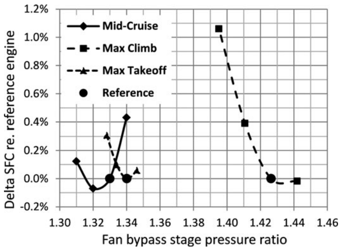
Figure 6. Effect of fan pressure ratio on SFC.
