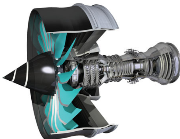
Figure 3. (Colour online) Rolls-Royce UltraFan ® engine concept having a variable-pitch geared fan.
