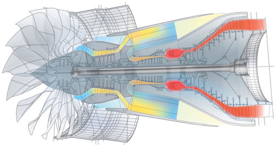
Figure 1. (Colour online) Schematic diagram of an intercooled engine with a low-speed LP turbine and a direct-drive fan.
