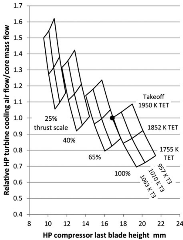
Figure 13. The effect on reference engine cooling flows of thrust scaling with different T_3 and TET limits at hot-day take-off vs HP compressor last blade height.
