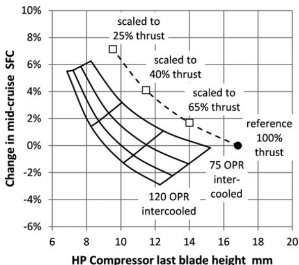
Figure 19. Improvements in mid-cruise SFC for intercooled engines from Fig. 18 with optimised mid-cruise intercooler effectiveness, OPR and TET vs the best conventional engines.
