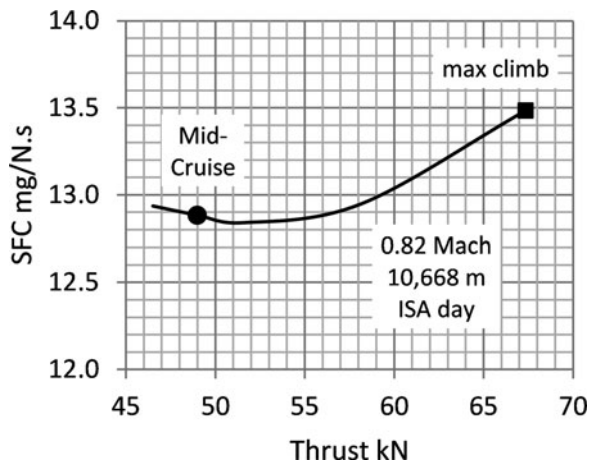
Figure 5. Reference 2050 turbofan SFC loop.
