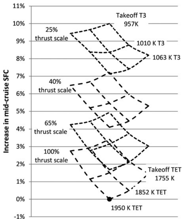
Figure 12. The effect on mid-cruise SFC of scaling the reference engine and designing it for various hot-day take-off temperature limits for T_3 and TET.
