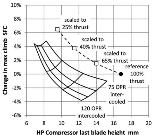
Figure 18. Effect of HP compressor last blade height and max climb OPR on max climb SFC for engines with 75% intercooler effectiveness vs the best conventional engines.
