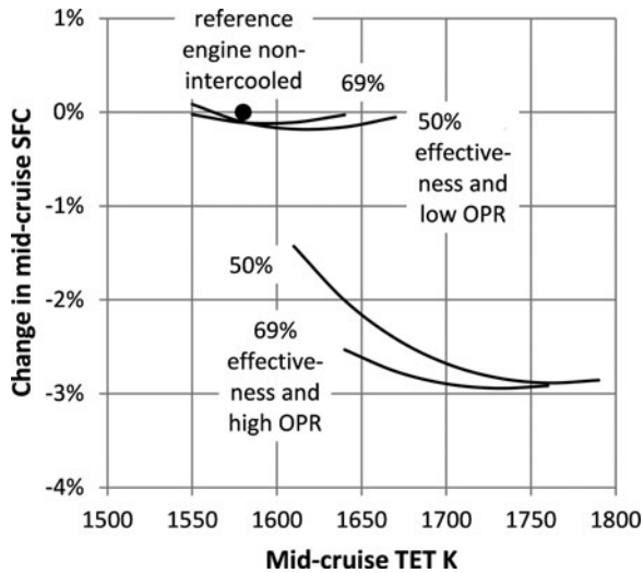
Figure 17. How mid-cruise SFC varies with TET and intercooler effectiveness for two different engines with 75 and 120 OPR at the max climb design point.
