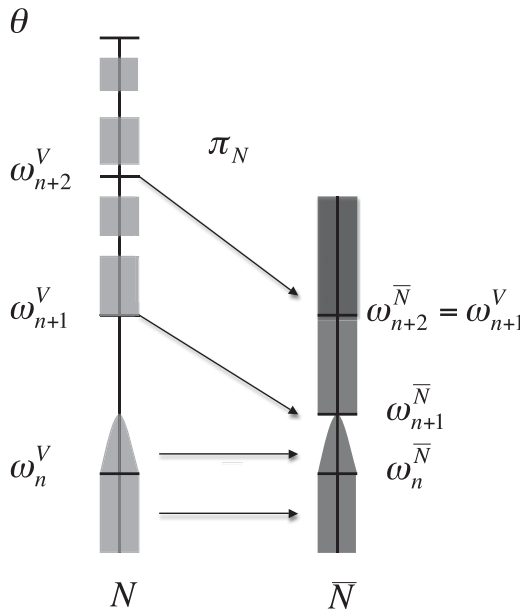
FIGURE 1. Proposition 2.1.
