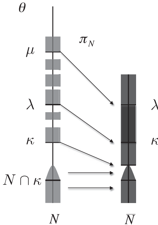
FIGURE 3. Example 2.6.
