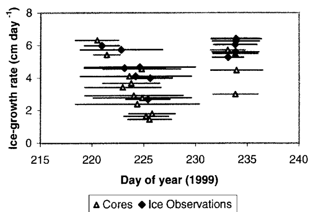
Fig. 3. Comparison of ice-growth rates from core samples (open triangles) and level-ice ship observations (solid diamonds). The lines indicate the range of dates from when the buoy was deployed in open water to the time the data on ice thickness were collected. Symbols are located at the midpoint of this time period.
