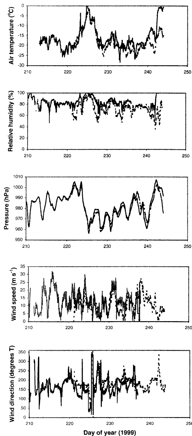
Fig. 2. Meteorological data collected during the experiment. The solid line is data collected on the ship; the dotted line is data collected from an automatic weather station located on Eder Island at 66° 57.5' S, 143° 56.5' E.
