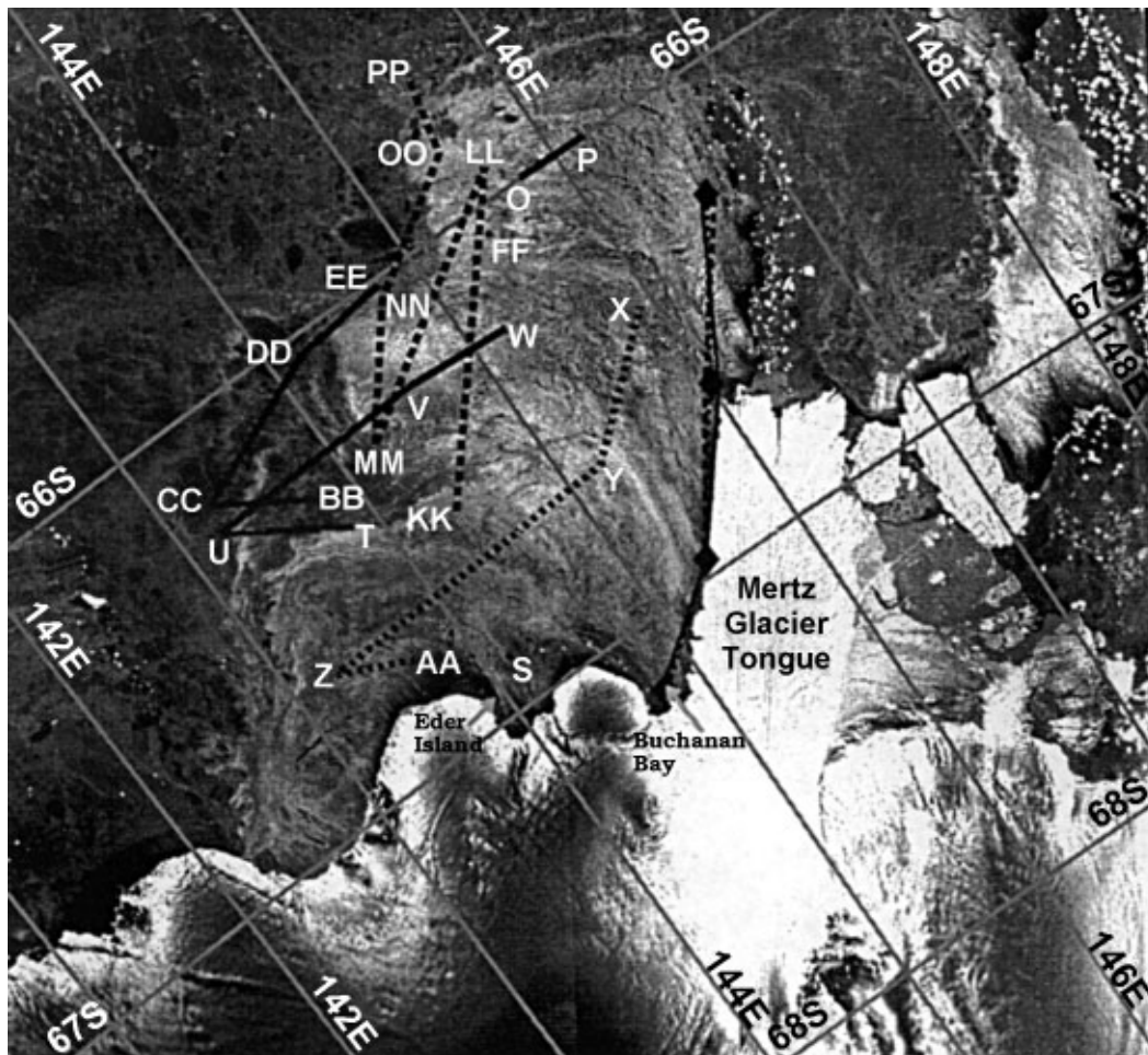
Fig. 1. RADARSAT SAR image collected on 4 August 1999. The initial deployment locations of the buoys are indicated with diamonds. Locations of each of the buoy revisits are indicated with the station name in capital letters. The ice-observations transects used for estimating ice-growth rates are shown drawn between the revisit locations. Array 1 is shown as a solid line, array 2 as a dashed line, and array 3 as a dotted line. SAR image © RADARSAT International, 1999.
