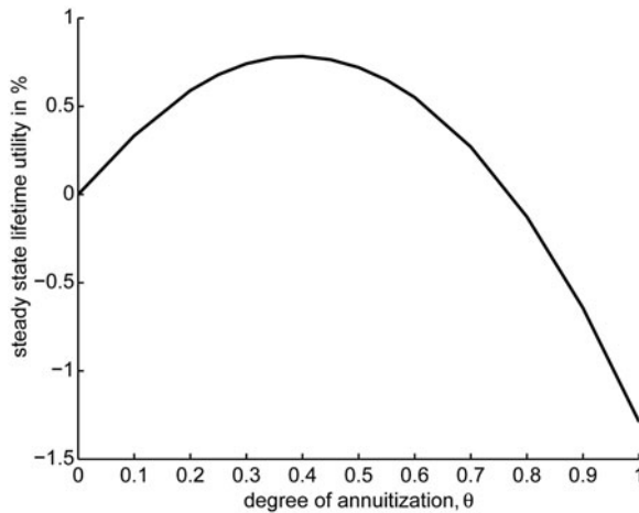
Figure 5. Optimal \theta .
