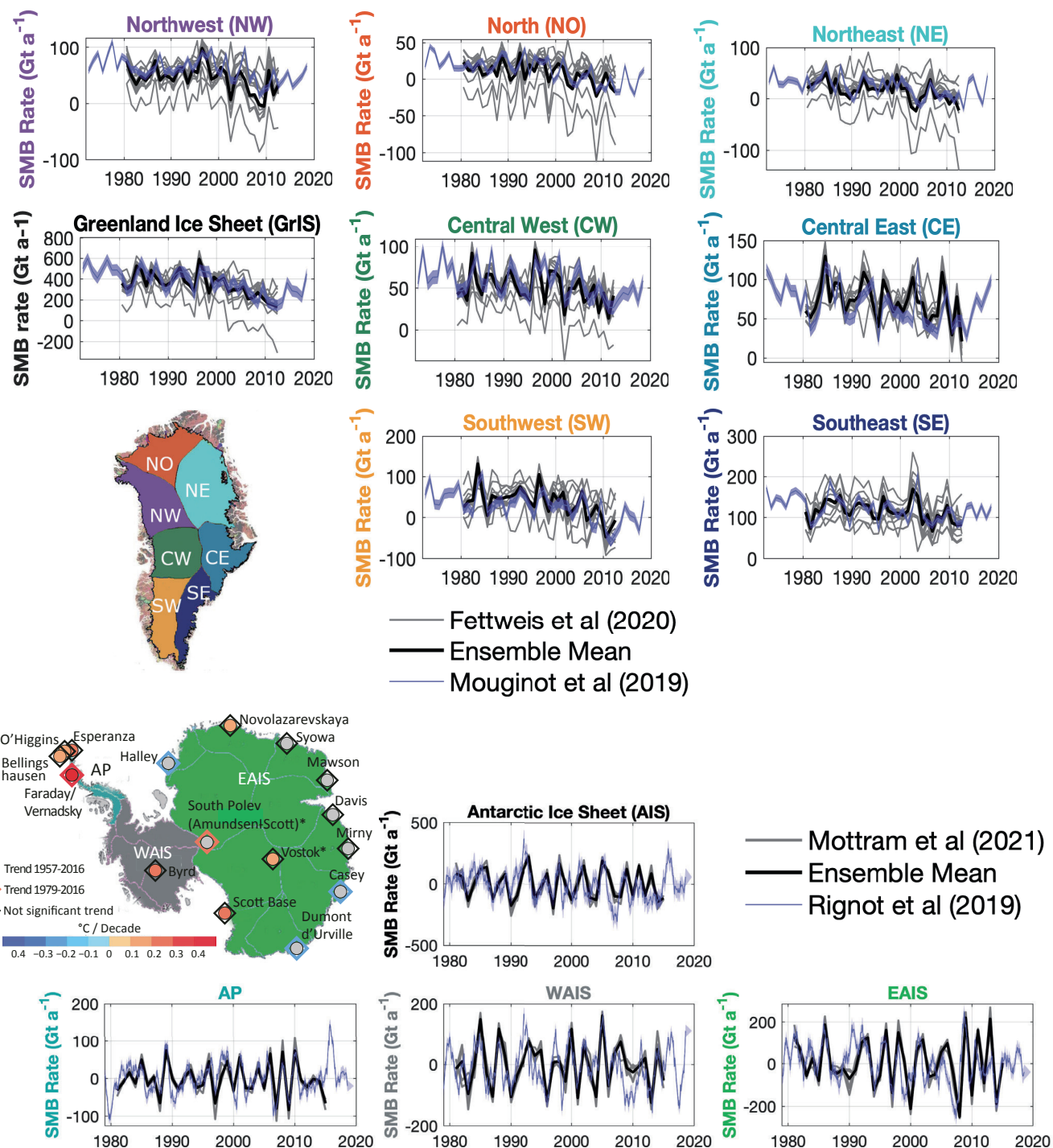
Figure Atlas.30 | (Upper panels) Time series of annual surface mass balance (SMB) rates (in Gt a -1 ) for the Greenland Ice Sheet and its regions (shown in the inset map) for the periods 1972–2018 (Mouginit et al., 2019) and 1980–2012 (Fettweis et al., 2020) using 13 different models. (Lower panels) Time series of annual SMB rates (in Gt a -1 ) for the grounded Antarctic Ice Sheet (excluding ice shelves) and its regions (shown in the inset map) for the periods 1979–2019 (Rignot et al., 2019) and 1980–2016 (Mottram et al., 2021) using five Polar-CORDEX regional climate models. The Antarctic inset map also shows the location of the stations discussed in Atlas.11.1.2 where observations are available for at least 50 years. Colours indicate near-surface air temperature trends for 1957–2016 (circles) and 1979–2016 (diamonds) statistically significant at 90% (Jones et al. 2019; Turner et al. 2020). Stations with an asterisk (*) are where significance estimates disagree between the two publications. Further details on data sources and processing are available in the chapter data table (Table Atlas.SM.15).
