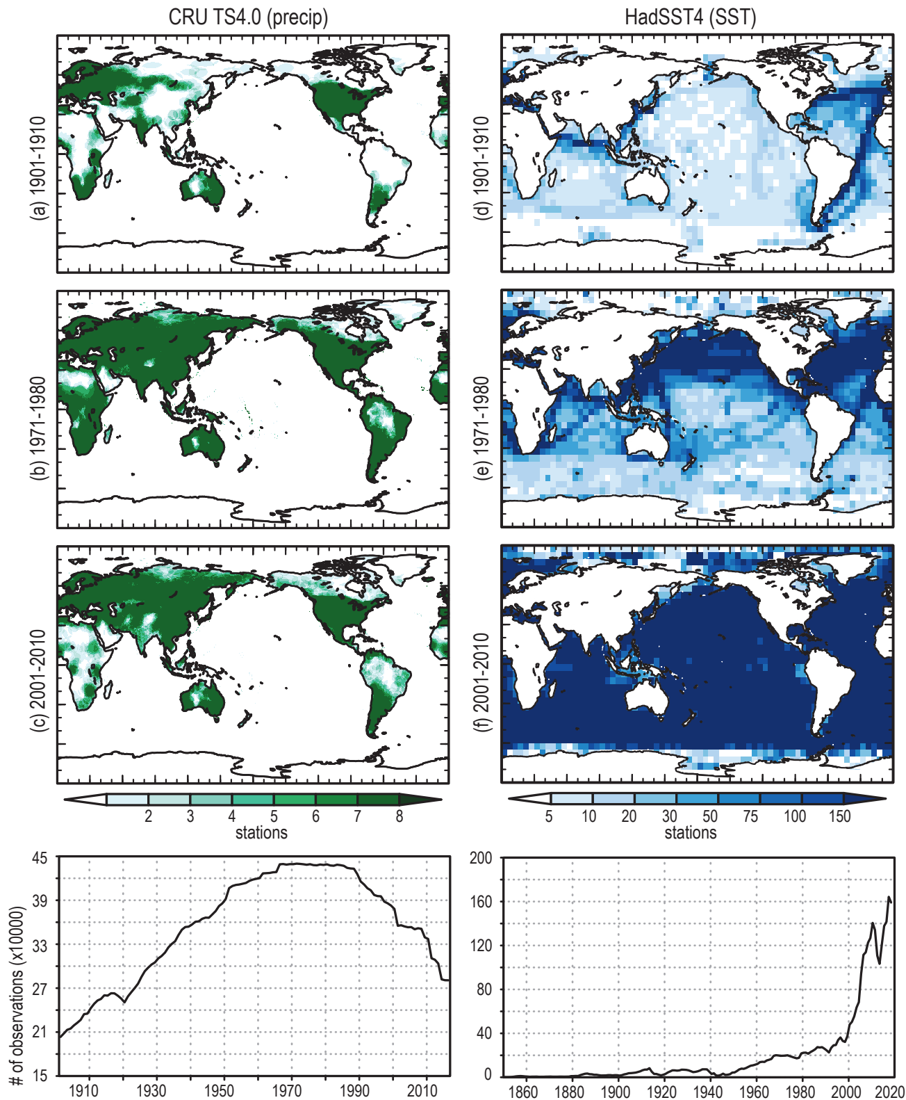
Figure Atlas.5 | Number of stations per 0.5^{\circ} \times 0.5^{\circ} grid cell reported over the periods of 1901–1910, 1971–1980, and 2001–2010 (rows 1–3), and the global total number of stations reported over the entire globe (bottom row) for precipitation in the CRU TS4 dataset (left) and the HadSST4 dataset (right). Further details on data sources and processing are available in the chapter data table (Table Atlas.SM.15).
