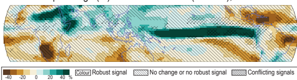
CMIP5 – Precip. change (%) for JJA 2081-2100 (RCP8.5), rel. to 1995-2014
