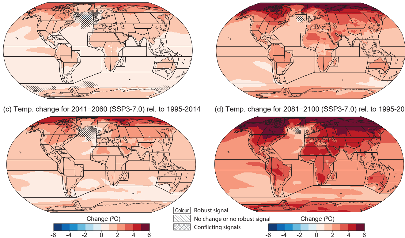
(a) Temp. change for 2041–2060 (SSP1-2.6) rel. to 1995–2014
