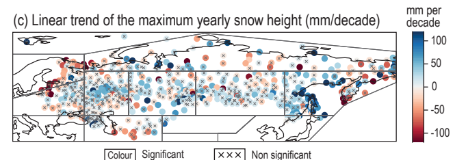
Figure Atlas.18 | Linear trends for the 1980–2015 period based on station data from the World Data Centre of the Russian Institute for Hydrometeorological Information (RIHMI-WDC; Bulygina et al., 2014). (a) Snow-season duration from 1 July to 31 December (days per decade); (b) snow-season duration from 1 January to 30 June (days per decade); (c) maximum annual height of snow cover (mm per decade). Trends have been calculated using ordinary least squares regression and the crosses indicate non-significant trend values (at the 0.1 level) following the method of Santer et al. (2008) to account for serial correlation. Further details on data sources and processing are available in the chapter data table (Table Atlas.SM.15).
