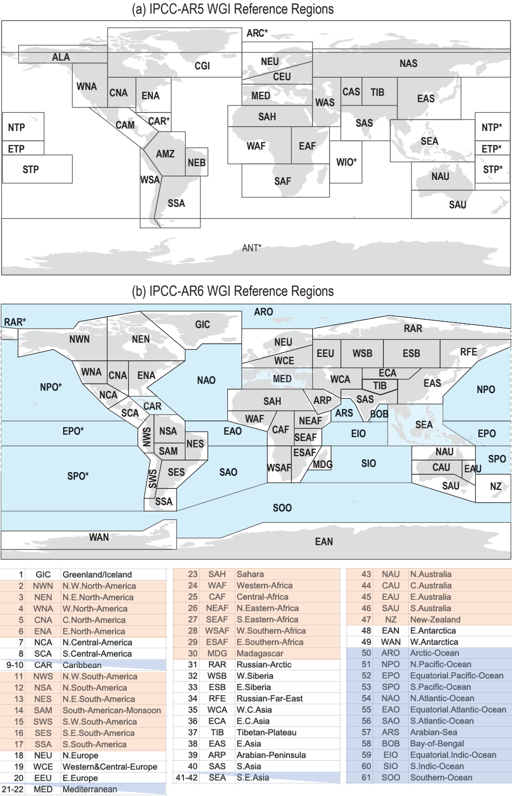
Figure Atlas.2 | WGI reference regions used in the (a) AR5 and (b) AR6 reports (Iturbide et al., 2020). Asterisks indicate regions that extend across both sides of the map.
