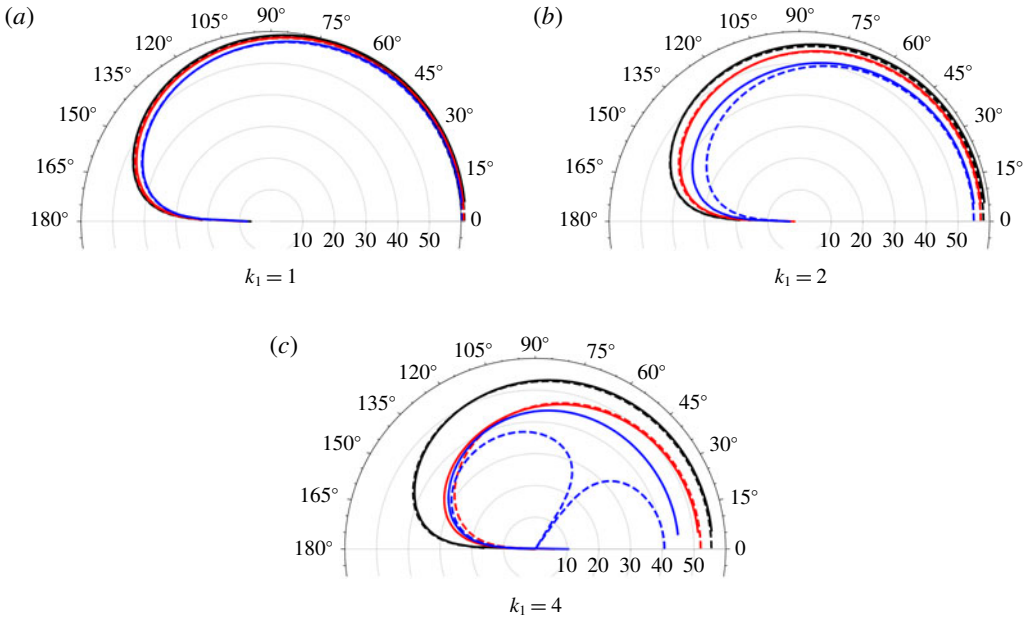
FIGURE 10. (Colour online) Polar plot of the (scaled) logarithmic spanwise-average directivity, 10 \log_{10}(10^8 D_{n,a}(r, \theta)) calculated numerically (solid) and analytically (dashed), for different serration height parameters: c = 0 (black), c = 2 (red), c = 4 (blue).
