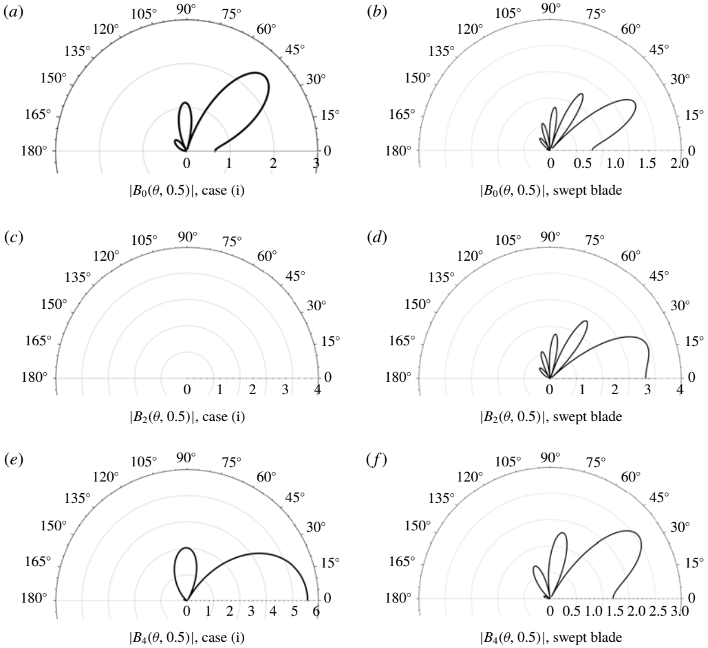
FIGURE 4. Polar plot of the magnitude of the n th mode, 10^4|B_n(\theta, z)| , as defined in (3.24), at mid-span point z = 0.5 , for M = 0.3 , k_3 = 0 , k_1 = 50 .
