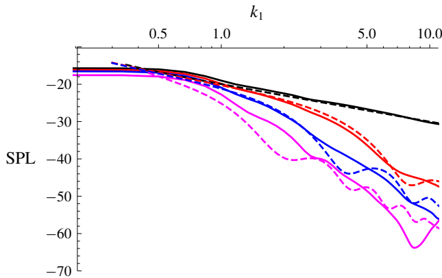
FIGURE 11. (Colour online) Comparison of the k_3 = 0 SPL calculated numerically for a line vortex (solid) and analytically for an incident gust (dashed), for c = 0 (black), c = 2 (red), c = 4 (blue), c = 8 (magenta).
