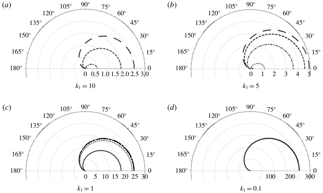
FIGURE 6. Polar plot of the spanwise-average directivity, 10^3 D_a(r, \theta) as given by (4.1), for case (ii) (periodic channel) with r = 10 , M = 0.3 , k_3 = 0 . Large dashed, c = 0 ; dashed, c = 0.5 ; dot-dashed, c = 1 ; dotted, c = 2 ; solid, c = 5 .
