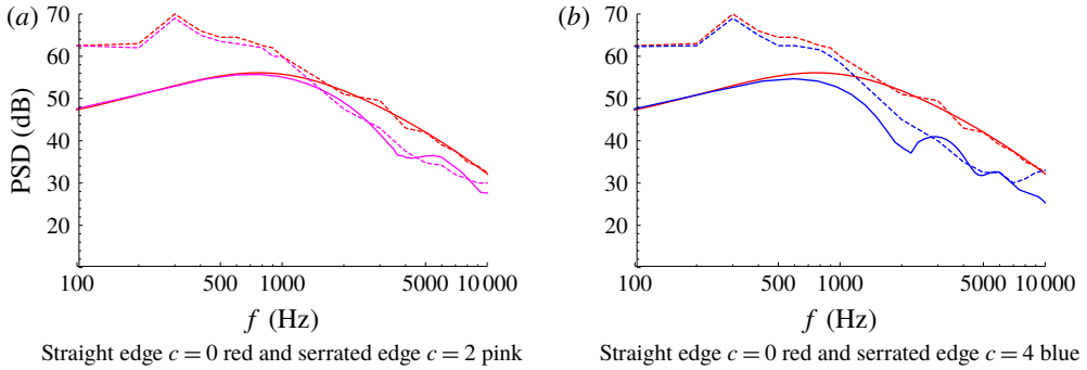
FIGURE 8. (Colour online) Comparison of far-field PSD for two serrated leading edges. Solid lines give the analytic results, dashed lines give the experimental measurements.
