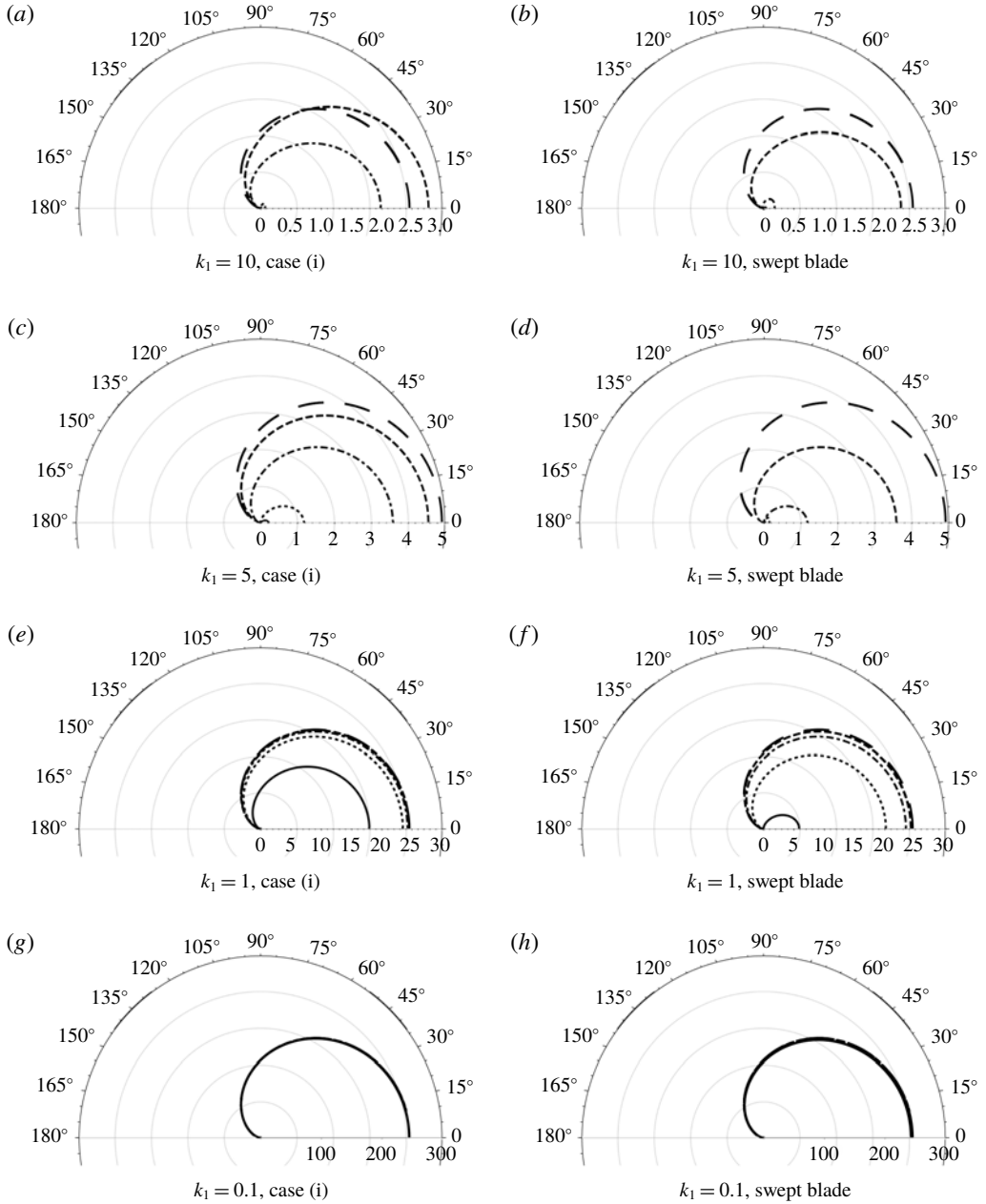
FIGURE 3. Polar plot of the spanwise-average directivity, 10^3 D_a(r, \theta) as given by (4.1), for r = 10 , M = 0.3 , k_3 = 0 . Large dashed, c = 0 ; dashed, c = 0.5 ; dot-dashed, c = 1 ; dotted, c = 2 ; solid, c = 5 .
