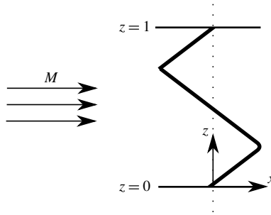
FIGURE 1. Uniform steady flow in the x direction with unsteady convective gust perturbation interacts with a rigid plate y=0 with serrated edge x=cF(z) .
