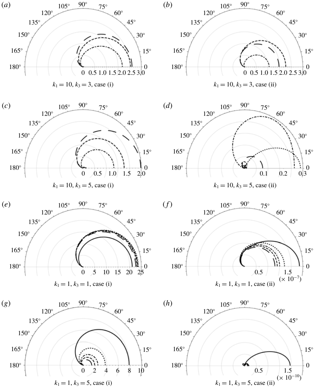
FIGURE 7. Polar plot of the spanwise-average directivity, 10^3 D_a(r, \theta) as given by (4.1), for r = 10, M = 0.3 . Large dashed, c = 0 ; dashed, c = 0.5 ; dot-dashed, c = 1 ; dotted, c = 2 ; solid, c = 5 .
