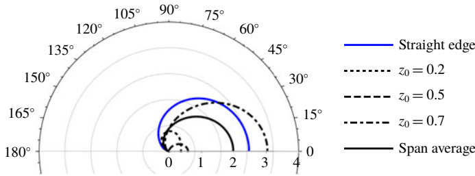
FIGURE 2. (Colour online) Polar plot of 10^3|p(10, \theta, z)|^2 compared to the span average, 10^3D_a(10, \theta) , and straight-edge, c=0 , results, for blades in a rigid-walled channel. In all cases M=0.3 , k_3=0 , k_1=10 . Serrated blades have c=1 .
