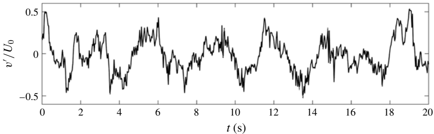
FIGURE 7. Time series segment of the measured (—) and interpolated ( \cdots ) values of v'/U_0 corresponding to the sample point in figure 6.
