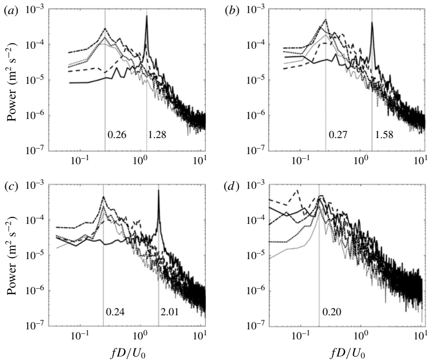
FIGURE 9. Single-point spectra of the velocity fluctuations ( v' ) taken at X/D = 0.9 (—), X/D = 1.7 (---), X/D = 3.3 (-·-·-), X/D = 7.3 (- - - - -), and X/D = 10.0 (· · · · ·). The spectra correspond to load-free shaft conditions for the (a) 2-bladed VAWT, (b) 3-bladed VAWT, (c) 5-bladed VAWT and (d) cylinder. Dotted vertical lines correspond to the selected near- and far-wake frequencies of the maximum amplitude in the spectra.
