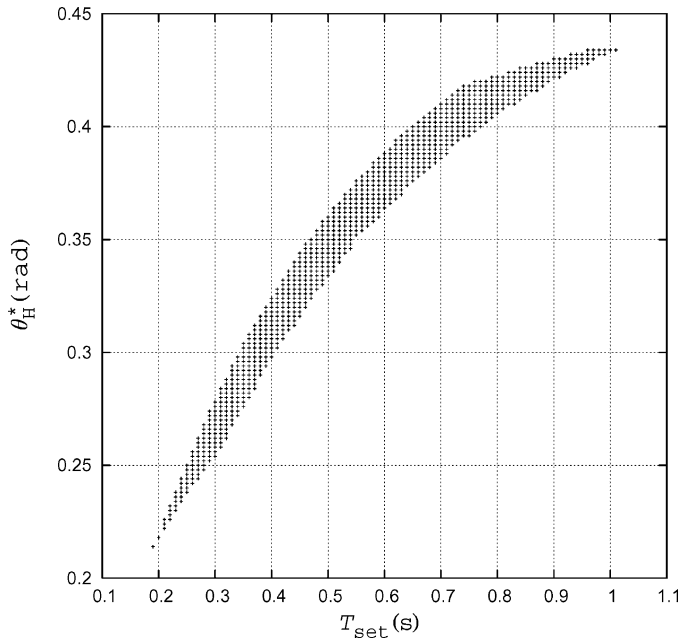
Fig. 11. Stable domain in T_{\text{set}}-\theta_H^* plane for virtual passive dynamic walking for \phi = 0.02 (rad).
