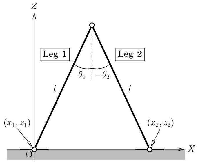
Fig. 4. Configuration at instant of heel strike.
