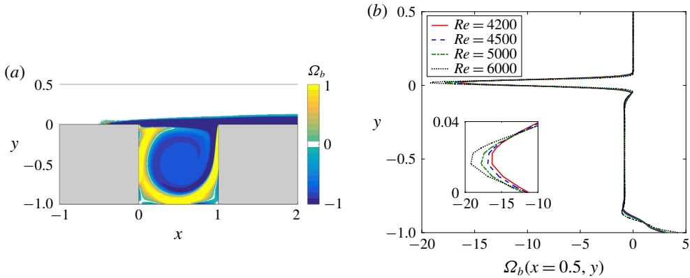
FIGURE 5. (Colour online) Stationary solution (base flow). (a) \Omega_b over the domain for Re = 4500 . (b) Vorticity profiles \Omega_b(x = 0.5, y) for Re = 4200, 4500, 5000, 6000 . The major change in the base flow with Reynolds number is localized on the shear layer region and at the bottom of the cavity.
