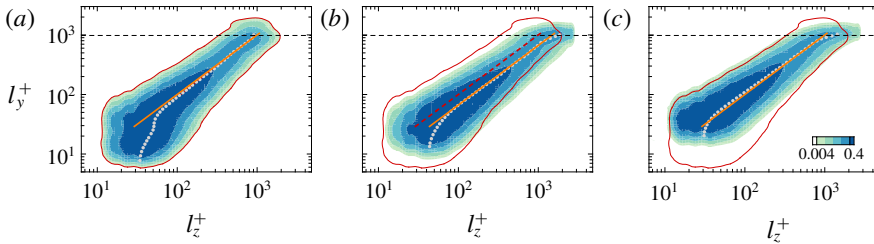
FIGURE 5. (Colour online) Joint PDFs of the logarithms of the width ( l_z ) of the attached structures and of their height ( l_y ): (a) u , (b) w and (c) v . The inserted dots indicate the mean l_z with respect to l_y . The orange solid lines are l_z^+ = l_y^+ in (a), l_z^+ = 1.5l_y^+ in (b) and l_z^+ = l_y^+ in (c). In (b) and (c), the red contour line represents the contour level of 0.004 in (a). The red dashed line in (b) is consistent with the orange line in (a). The horizontal dashed line indicates l_y^+ = \delta^+ . The contour levels are logarithmically distributed.
