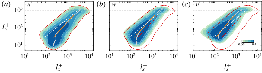
FIGURE 4. (Colour online) Joint PDFs of the logarithms of the length ( l_x ) of the attached structures and of their height ( l_y ): (a) u , (b) w and (c) v . The inserted dots indicate the mean l_x with respect to l_y . The orange solid lines are the best fit, l_x^+ \sim (l_y^+)^{\gamma} of the data for 100 < l_y^+ < 550 ; l_x^+ = 17.98(l_y^+)^{0.74} in (a), l_x^+ = 12.10(l_y^+)^{0.74} in (b) and l_x^+ = 11.34(l_y^+)^{0.69} in (c). In (b) and (c), the red contour line represents the contour level of 0.004 in (a) and the red dashed line is consistent with the orange line in (a). The white dashed line ( l_x^+ = 3l_y^+ ) indicates the scaling of the vortex and Reynolds shear stress clusters (del Álamo et al. 2006; Lozano-Durán et al. 2012). The horizontal dashed line indicates l_y^+ = \delta^+ . The contour levels are logarithmically distributed.
