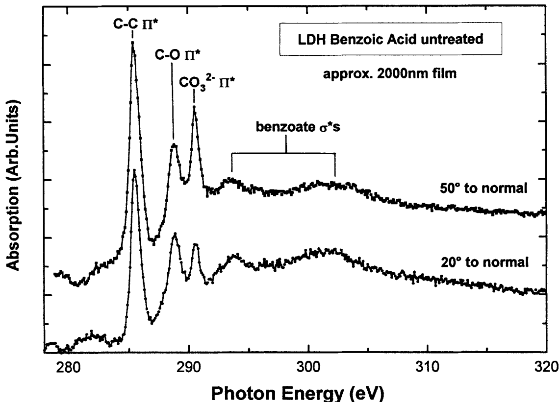
Figure 6. Background subtracted NEXAFS spectra of an approximately 2000 nm LDH Benzoate film (dried in air), normalized to the carbon atomic absorption. Recorded in fluorescence mode.
