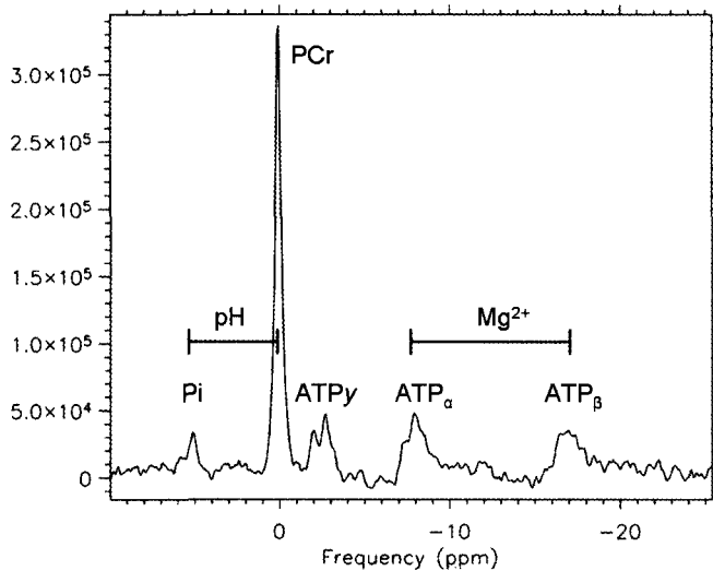
Figure 6: A typical ^{31}\text{P} -MRS spectrum with measured metabolites indicated. From G. Wells, 2007 (unpublished results).
