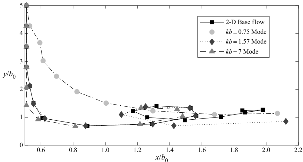
FIGURE 13. A comparison of the trajectories of the nonlinear evolution of the primary vortices for the various optimal perturbations. The solid line (-) shows the trajectory of the primary vortex for the 2-D base flow case, the dash-dot (-.-) line shows the trajectory of the long-wavelength mode kb = 0.75 for A = 0.0002 , illustrating the suppression of the vortex rebound. The dotted line ( \cdots ) shows the trajectory for the kb = 1.57 mode and A = 0.0002 , and the dashed line (- -) shows the kb = 7 , A = 0.0002 trajectory.
