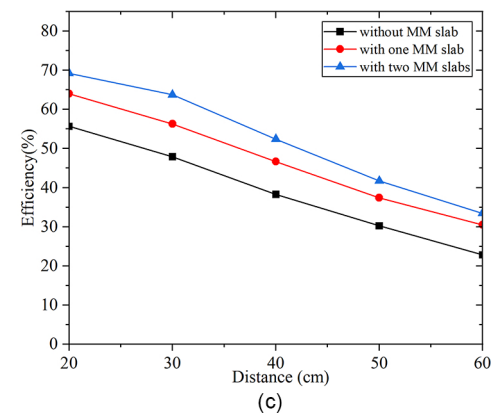
Figure 14. PTEs of MCR-WPT system with two MM slabs: (a) in the middle, (b) near the Tx coil, and (c) near the Rx coil.
