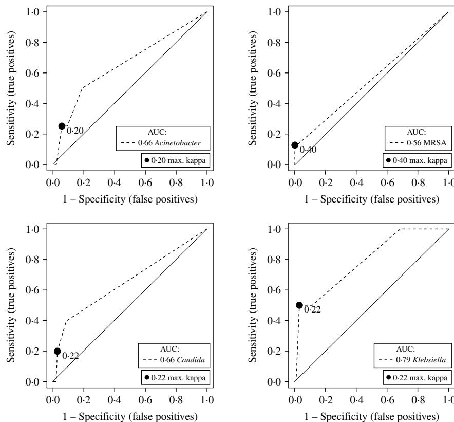
Fig. 4. Receiver operator characteristic (ROC) plots assessing model performance for the four parsimonious path models when used to predict outcomes in the validation dataset. Note that the models used the direct effects and not indirect effects of variables, since the endogenous proximal variables in the networks were all directly observed.
