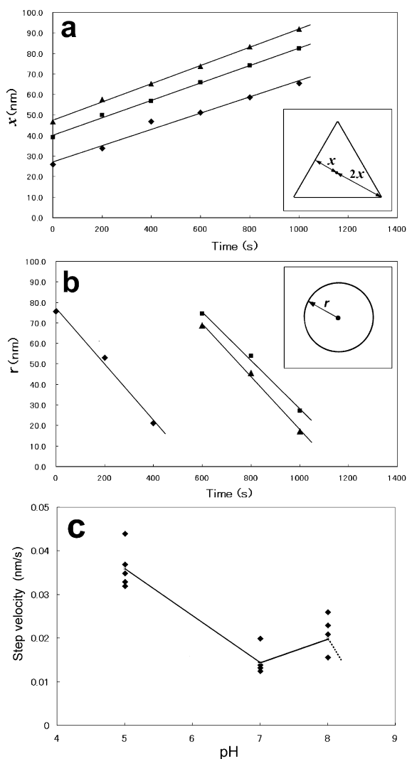
Figure 5. (a) The size of the triangular etch pits in Figure 1a as a function of time. The vertical axis is the distance from the center of the triangle to the side ( x ), which is calculated from the area of the triangle measured from AFM images. The three regression lines represent the different pits and the slopes of these lines correspond to the step velocity. (b) The sizes of the stranded terraces in Figure 1a with time. The vertical axis represents the radius of the circle with the same area as the terrace. (c) pH dependence of the step velocity around the triangular etch pits. The plots at pH 7 represent the result using de-ionized water.
