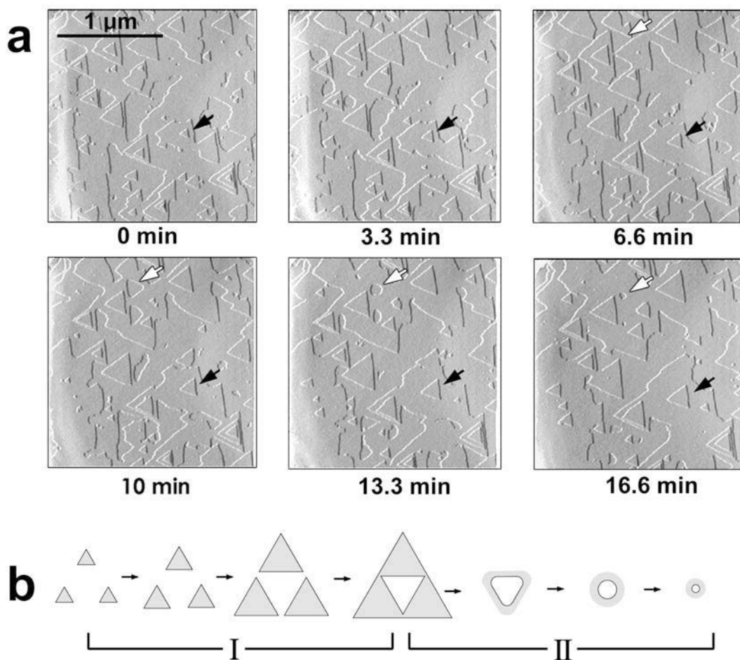
Figure 1. (a) AFM images showing the surface microtopography of brucite in solution at pH 5. These images and those in the other figures are expressed by differential mode. The step height is 0.5 nm and this height corresponds to the monolayer thickness of \text{Mg}(\text{OH})_2 . The black arrow indicates the same triangular etch pit in each image, expanding in size with time. The white arrow shows a stranded terrace formed by the coalescence of etch pits, diminishing in size with time. (b) A diagram to show the dissolution process of brucite on the (001) surface. Triangular etch pits form and expand until they coalesce (I). A stranded terrace forms by the coalescence of the pits and diminishes in size with a rounded shape (II).
