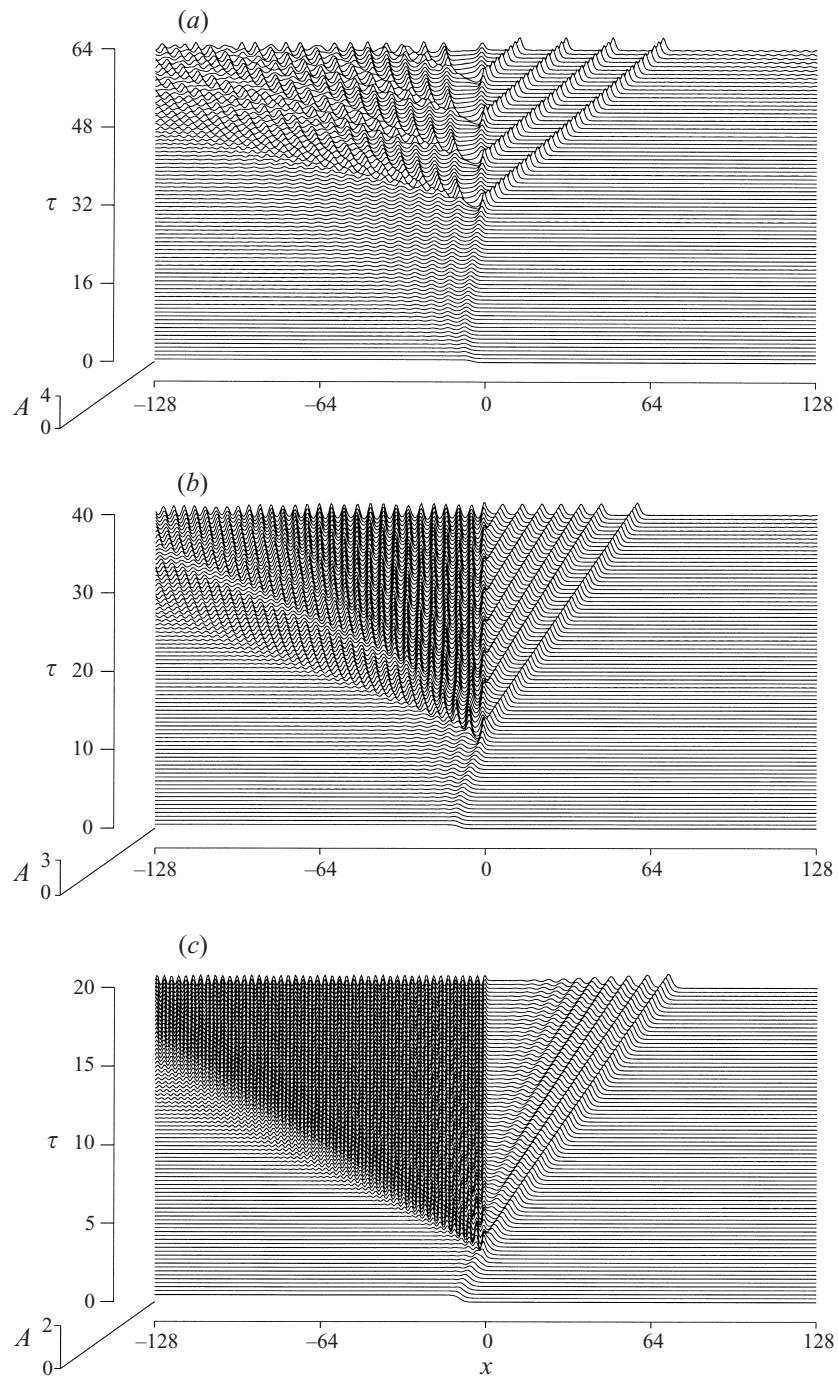
FIGURE 5. Three solutions of (2.25), (2.26) and (2.27) for A = 1/3 , x_a = 1/2 and \Delta_1 = 2 , corresponding to a solution from each of the regimes in figure 4. (a) A strong resonance solution where \Delta_0 = -1 ; (b) a unsteady weak resonant solution where \Delta = 0 and in (c) a subcritical or steady weak solution where \Delta_0 = 3 .
