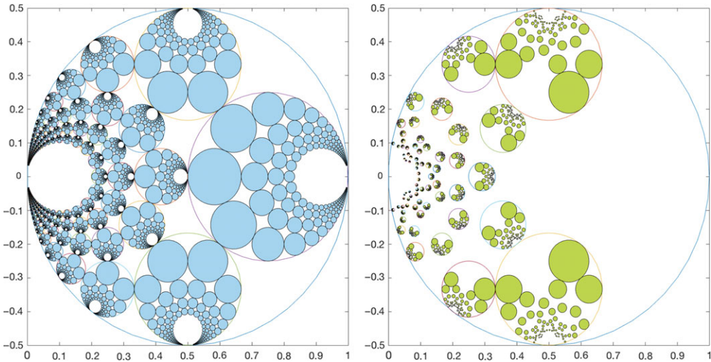
Fig. 1. Approximation of the limit sets \mathcal{C}\mathcal{F}_E and of \mathcal{C}\mathcal{F}_{GP-\pi,\pi} after two iterations.
