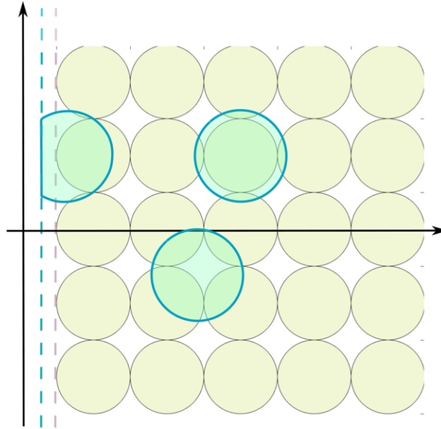
Fig. 2. The grid of balls \cup_{e \in E} \overline{B}(e + 1/2, 1/2) and examples of the sets C(z, 1/2 + r) for z \in H_1^+ and r \leq 4\eta .
