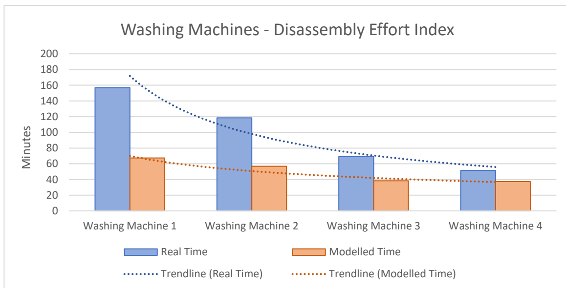
Figure 7. Washing Machine DEI; The modelled time is obtained using the modified MOST; Real time is obtained using a stopwatch
