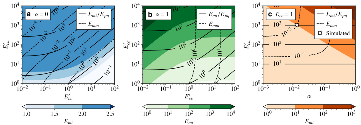
Fig. 2. Bulk enhancement factors E_{mt} (coloured contours), E_{mmm} (dashed contours), and E_{mt}/E_{pq} (solid contours) for a unidirectional orientation fabric ( \mathbf{c} = \mathbf{m} ) as a function of the grain enhancement factors E'_{cc} and E'_{ca} in the case of (a) the Sachs model, (b) the Taylor model, and (c) a linear combination of the Sachs and Taylor models depending on \alpha (assuming grains are equally hard to compress along \mathbf{c} and \mathbf{a} , implying E'_{cc}=1 ). The cross in panel c indicates the grain parameters used to model the bulk enhancement factors in our ice-flow simulations. Note the colourbar scale is linear in panel a, as opposed to in panel b and panel c, because E_{mt} varies less in the Sachs model (see main text).
