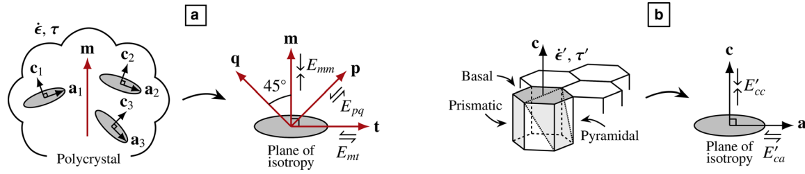
Fig. 1. (a) Axisymmetric polycrystal with longitudinal ( E_{mm} ), shear ( E_{mt} ), and 45^\circ -shear ( E_{pq} ) bulk enhancement factors with respect to the symmetry axis \mathbf{m} . The transverse direction, \mathbf{t} , lies in the plane of isotropy ( \mathbf{t} \perp \mathbf{m} ), while \mathbf{p} is oriented at 45^\circ to \mathbf{m} and \mathbf{p} \perp \mathbf{q} . (b) Monocrystal lattice composed of hexagonal cells. Three crystallographic planes are highlighted in grey, where the c -axis indicates the basal-plane normal direction. Monocrystals are modelled as a transversely isotropic material with symmetry axis \mathbf{c} and longitudinal ( E'_{cc} ) and shear ( E'_{ca} ) enhancement factors with respect to \mathbf{c} . The transverse direction, \mathbf{a} , lies in the plane of isotropy ( \mathbf{a} \perp \mathbf{c} ).
