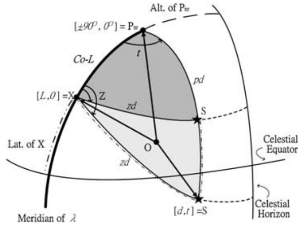
Figure 4. An astronomical triangle in the combined celestial equator and celestial horizon systems of coordinates.
