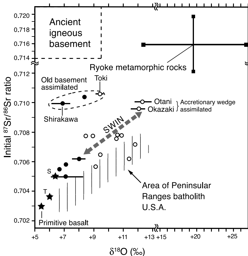
Figure 8 Initial ^{87}\text{Sr}/^{86}\text{Sr} ratio versus \delta^{18}\text{O} ratios of the late Cretaceous–Palaeogene batholith of the Inner Zone of SW Japan (SWIN). Revised from Ishihara & Matsuhisa (2002). The original data for the Peninsular Range batholith are taken from Taylor (1986). (solid circle) magnetite series; (open circle) ilmenite series; (star with S) Palaeocene gabbro in Shimane Prefecture; (star with T) Miocene gabbro in Tanzawa; (primitive basalt) Quaternary tholeiitic basalt of Hachijo-jima (Matsuhisa et al. 1973).
