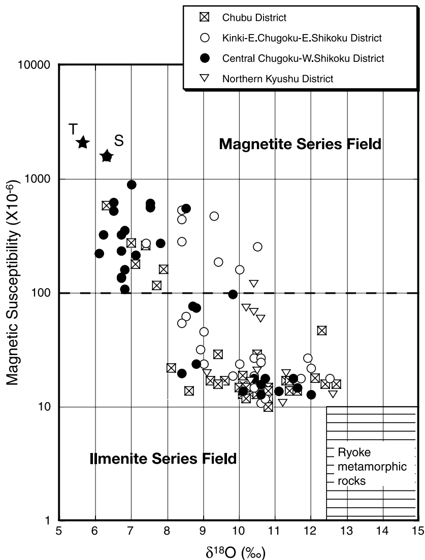
Figure 7 Magnetic susceptibility versus \delta^{18}\text{O} values of the late Cretaceous–Palaeogene granitoids, SW Japan. The granitoids plot between the gabbroids of the Miocene Tanzawa body (star with T) and those of the Palaeogene body in Shimane Prefecture (star with S), and Jurassic accretionary wedges of the Ryoke metamorphic rocks. The original data from Ishihara and Matsuhisa (2002). Several granitoids which have possibly interacted with meteoric water in the Sanyo Belt are excluded.
