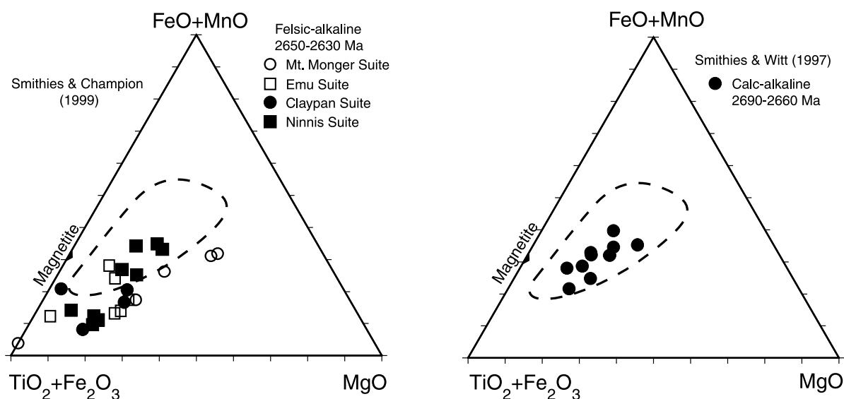
Figure 13 Bulk femic compositions of the Archaean granitoids, Eastern Goldfield, Yilgarn Craton, Western Australia. The felsic alkaline granitoids are extremely oxidised. Data sources: Smithies & Witt (1997); Smithies & Champion (1999). The broken circle shows the representative area of the magnetite-series granitoids of the Sanin Province, Japan.
