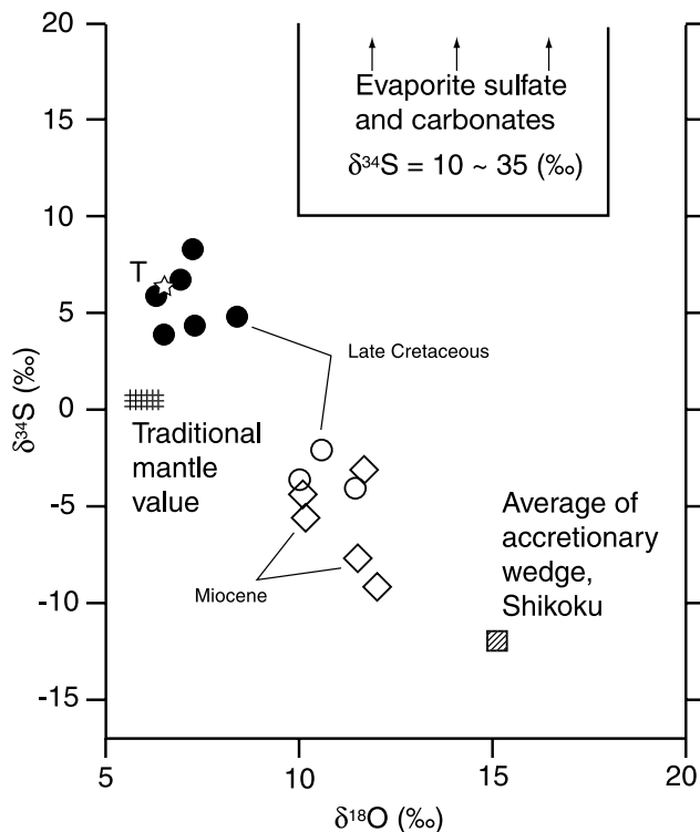
Figure 5 Whole rock \delta^{34}\text{S} versus \delta^{18}\text{O} values of the late Cretaceous to Miocene granitoids in SW Japan. (star with T) Tanzawa tonalite; (solid symbols) magnetite series; (open symbols) ilmenite series. Note that the SW Japan granitoids have no relationship with the sulphate-sulphur of evaporite and carbonates, which is common in the Cino-Korean Paraplatform (Ishihara et al. 2002a), but with that of the biogenic sulphur from the accretionary complexes.
