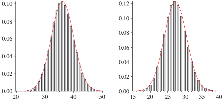
FIGURE 2: Histograms of the distribution of the number of symmetrical nodes in trees of size 100, compared to a matching Gaussian. Left: Otter trees of \mathcal{U}_{100} . Right: phylogenetic trees of \mathcal{B}_{100} .
