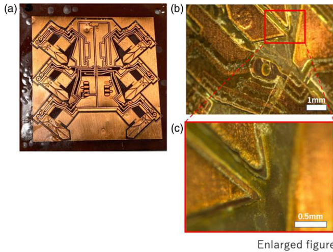
Figure 10. MEMS process. (a) SU-8 board. (b)(b) Leg tips and wiring area. (c) Enlarged view of leg tips.
