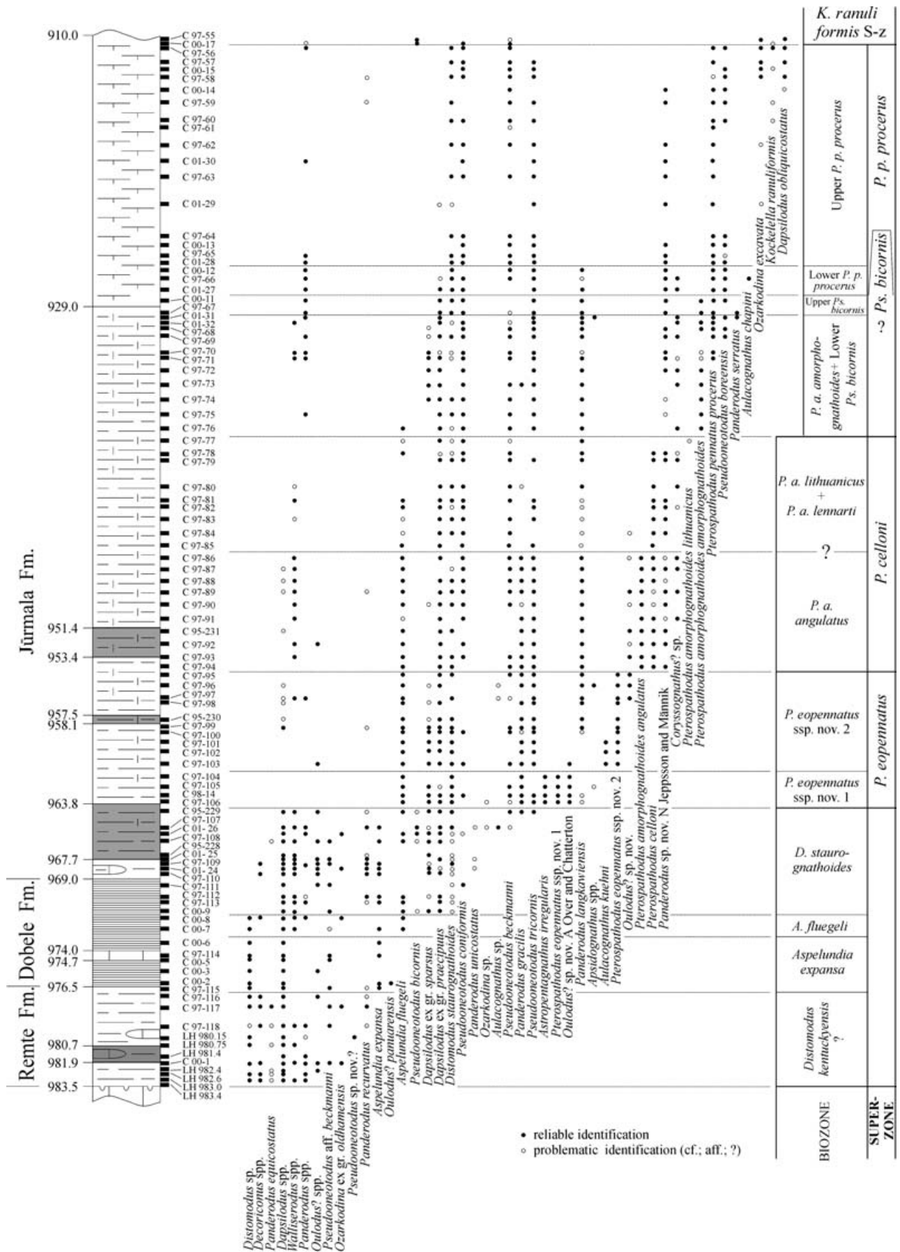
Figure 13. Range chart for conodonts through the Aizpute-41 core. For lithological legend see Figure 2.
