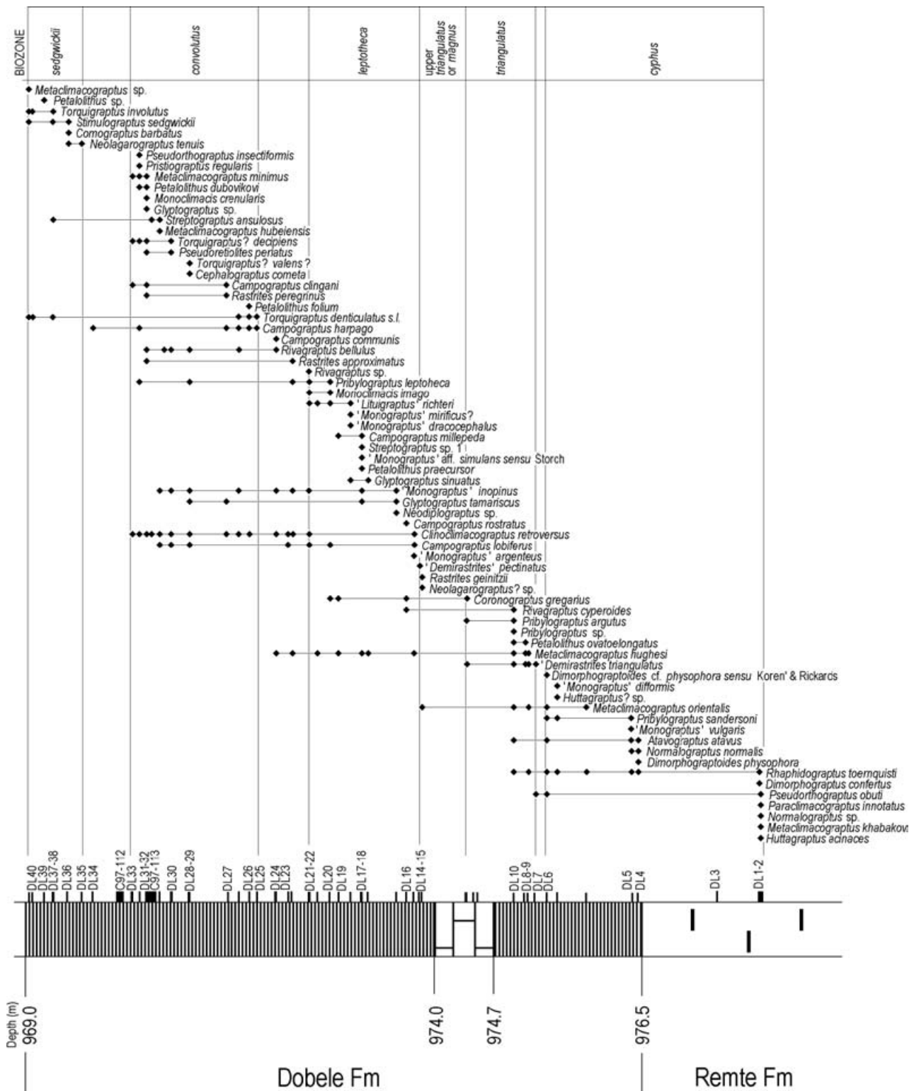
Figure 10. Range chart for graptolites through the Rhuddanian and Aeronian of the Aizpute-41 core. For lithological legend see Figure 2. In the BIOZONE column, boxes left blank indicate that the strata at this level could belong in either of the named biozones, above or below.
