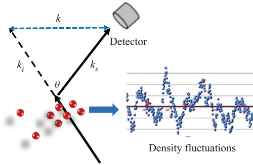
FIGURE 1. Schematic of the spontaneous RBS process, where the light is scattered by the spontaneous density fluctuations in the gas. The vectors k_i and k_s represent the incident and scattered light wave momentum vectors, respectively, while k represents the Brillouin scattering vector, in both directions for Stokes and anti-Stokes scattering. The scattering wavelength is L = \pi/|k_i| \sin(\theta/2) . Figure modified from figure 1(a) in Wu & Gu (2020).
