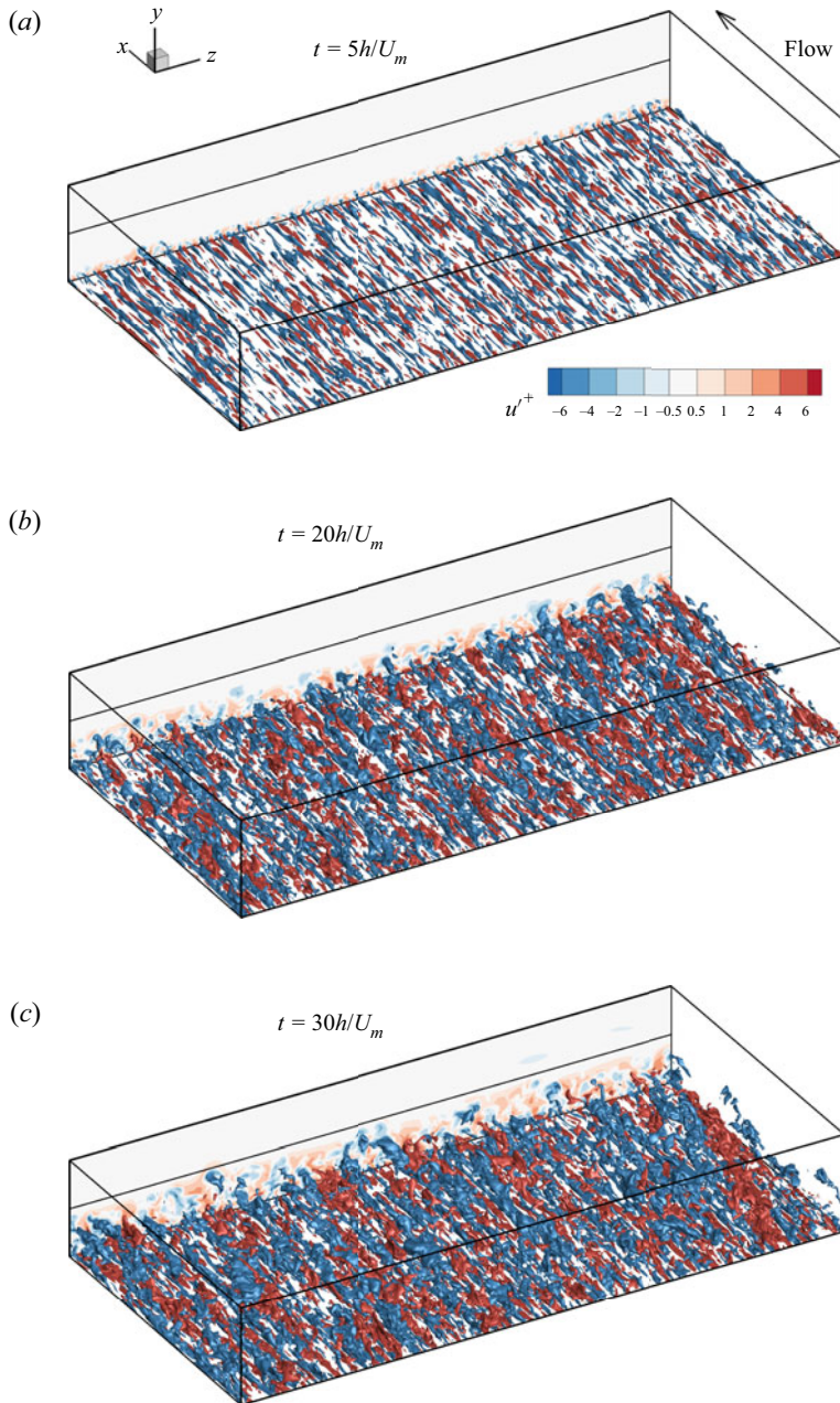
Figure 13. Distributions of u' in the lower half-channel at (a) t = 5 , (b) t = 20 and (c) t = 30 . Length in the x direction is 2\pi and in the z direction is 4\pi . Red: u'^+ = 3 ; blue: u'^+ = -3 . Flow is from bottom right to top left.
