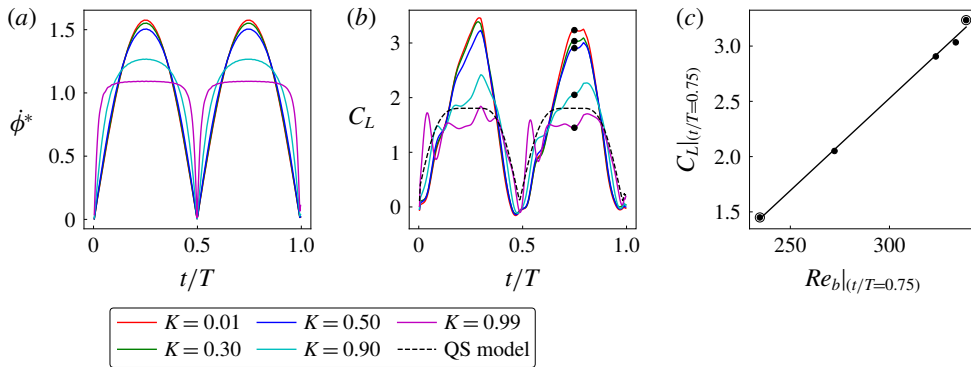
FIGURE 4. The phase-averaged time traces of (a) \dot{\phi}^* and (b) C_L with varying K . The dashed line in (b) indicates the predictions using the quasi-steady model of Sane & Dickinson (2002). The black dots in (b) represent the instantaneous values of C_L at t/T=0.75 , which (c) vary linearly with the instantaneous Reynolds number. The extreme cases, marked with open circles in (c), are discussed later in detail.
