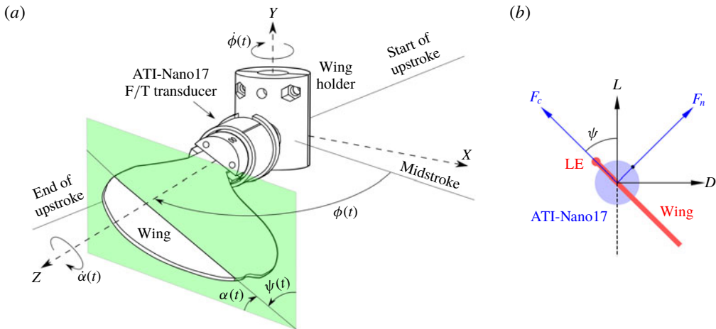
FIGURE 1. The schematics show (a) the flapping-wing set-up and (b) the alignment of the forces measured using an ATI-Nano17 F/T transducer attached to the wing root. The coordinates are shown in the wing's reference frame, where the Y axis is aligned with the sweep axis and the Z axis is aligned with the pitch axis along the wingspan.
