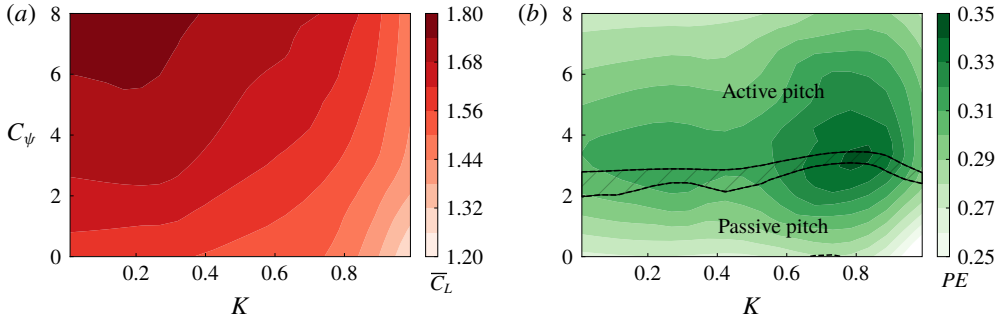
FIGURE 8. The contours of (a) \overline{C}_L and (b) PE on the K – C_\psi planes. The regions showing the feasibility of the passive and active pitch motions have been separated by a hatched transition region (due to the uncertainty in measurements) in (b).
