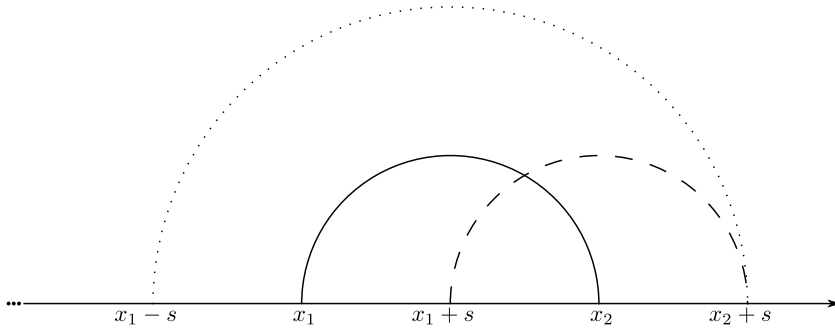
FIGURE B.1. The geometric meaning of the vectors (1, 1) and (-1, 1) considered in the proof of Proposition 6.3.
