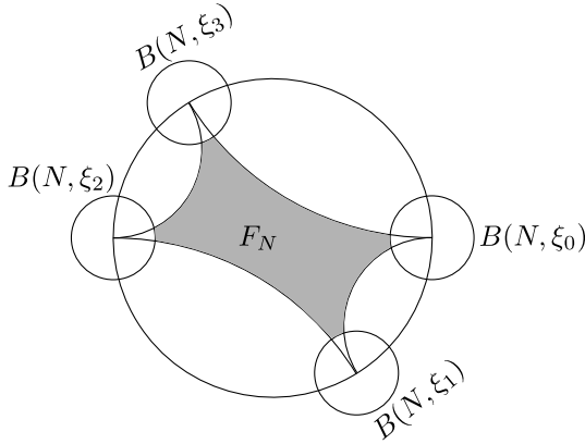
FIGURE 7. A schematic picture of the set F_N , in dark grey inside \mathcal{F} .
