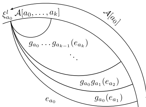
FIGURE 2. A left cuspidal word a_0 \cdots a_k .
