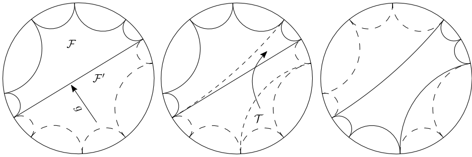
FIGURE 4. The surgery of the domain described in §3.1.
