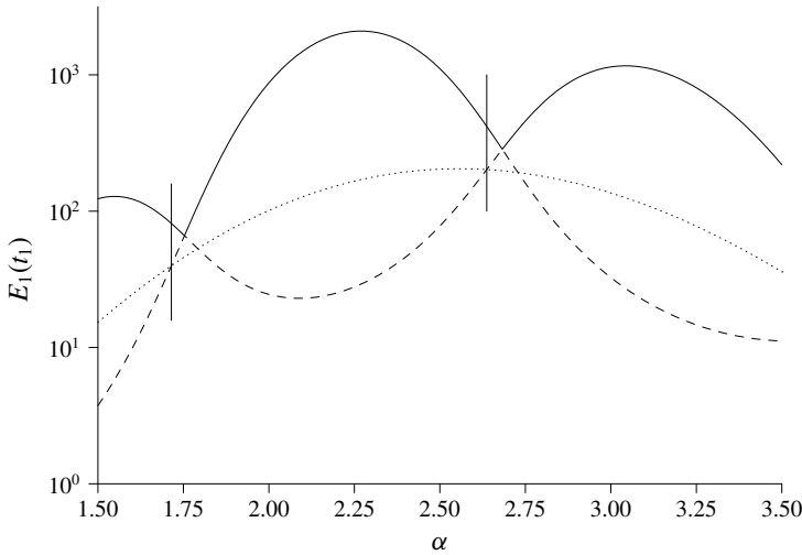
FIGURE 7. A comparison of the predicted growths of E_1(t_1) for Ra_T = 3000 and Ra_S = 2000 as a function of \alpha with \sigma = 7 , \tau = 1/80 and t_1 = 0.5 for conventional linear analysis (dotted line) and for the current approach optimized with respect to \lambda and \mu (solid line). The growth of the second mode is indicated by the dashed line. The vertical lines indicate where \omega t_1 = 3\pi and \omega t_1 = 4\pi respectively.
