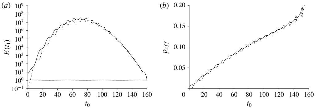
FIGURE 18. Graph of (a) E(t_1) and (b) p_{eff} , the effective growth rate, as t_0 is varied for a constant heat flux. Here R_\rho=1.8 , t_1=160 and \alpha=0.27 .
