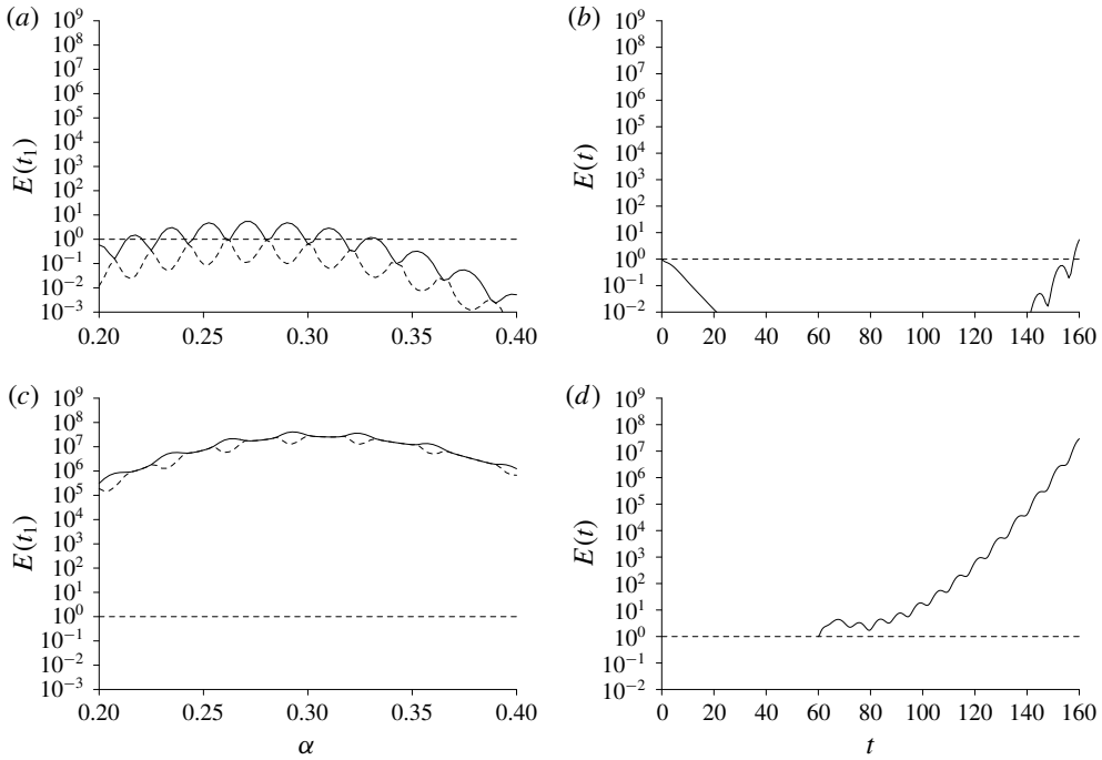
FIGURE 17. Graphs with t_0=0 and t_1=160 for R_\rho=1.8 and \alpha=0.27 of (a) E(t_1) as a function of \alpha and (b) the corresponding growth of the mode. The corresponding graphs with t_0=60 are shown in (c) and (d).
