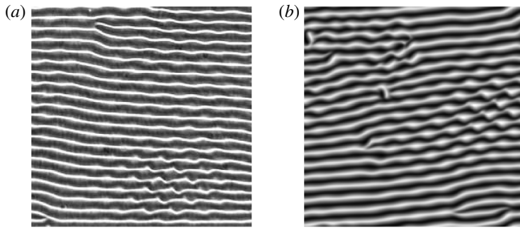
FIGURE 12. Snapshots of subharmonic oscillatory patterns (LSO) for Pr=1.07 , \gamma=17^\circ and \epsilon=1.5 from experiments (a) and from our numerical simulation (b).
