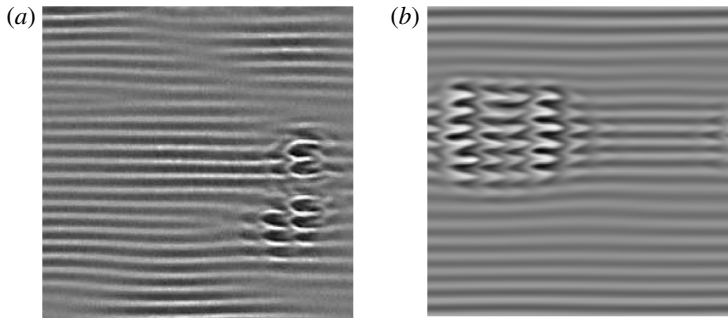
FIGURE 16. Localized transverse burst (TB) for the parameters Pr = 1.07 , \gamma = 77^\circ and \epsilon = 0.04 in experiments (a) and in simulations (b).
