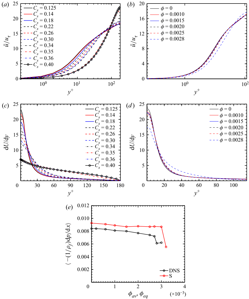
Figure 16. The streamwise mean velocity (a) for Re_b = 5600 , (b) Re_b = 5600 , St = 210.93 , mean velocity gradient (c) for Re_b = 5600 , (d) Re_b = 5600 , St = 210.93 , and pressure gradient (e) for Re_b = 5600 . The streamwise velocity in panels (a,b) are normalized with unladen frictional velocity ( u_\tau ). The mean velocity and pressure gradient in panels (c–e) are normalized with fluid bulk velocity and channel width. In panels (a,c), the simulations are performed with different C_s for the Smagorinsky model. Panels (b,d) show the results from particle-laden DNS for St = 210.93 . The pressure gradient for a range of \phi_{av} and \phi_{eq} is compared in panel (e) where the legend is S, Smagorinsky model and DNS, direct numerical simulation.
