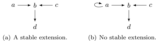
Fig. 1. Examples of argumentation frameworks.
