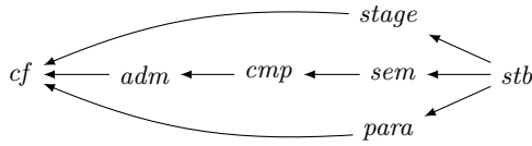
Fig. 5. Taxonomy of some argumentation semantics.
