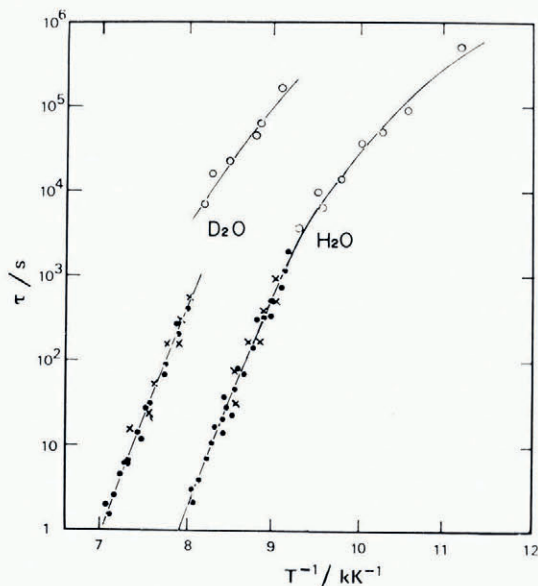
Fig. 4. Relaxation-time data of ice crystals determined by dielectric and calorimetric methods. ○ calorimetric method × TSD method, ● step-response (or bridge) method.
