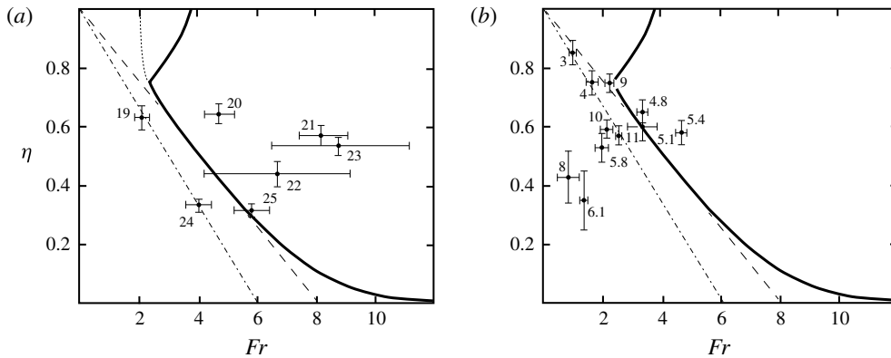
FIGURE 5. Values of \eta and Fr at numbered kilometre locations in the Samoan Passage (a) x=19 – 25 and (b) x=3 – 12 . Points to the right of the bold line are supercritical, those to the left subcritical. The uncertainties in observed values of \eta and Fr are shown by error bars. The dot-dashed line corresponds to an interfacial gradient Richardson number of 1/3 .
