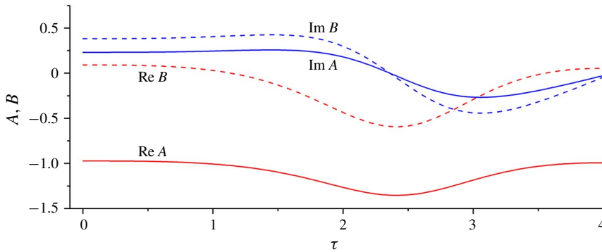
FIGURE 3. Evolution of A and B with \tau ; m = 1/2 , f = 4/3 , \mathcal{N} = 4/3 .
