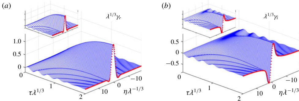
FIGURE 8. The analytical solution (6.6) for strong diffusion and A = -1 , showing (a) \lambda^{1/3}\gamma_r and (b) \lambda^{1/3}\gamma_i against the scaled space and time variables \lambda^{-1/3}\eta and \lambda^{1/3}\tau . The (red) dots show the final steady-state solution. The insets show corresponding numerical solutions to the reduced model, computed for \lambda = 5.3 .
