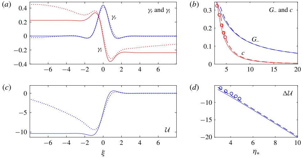
FIGURE 10. A coherent structure computed from (6.8) with \eta_* = 5.04 and A = -1.2 , showing (a) \gamma_r and \gamma_i , and then (c) \mathcal{U} (solid lines). The dotted lines show the numerical solution of the modified canonical model (6.4), computed for \lambda = 0.53 at \tau = 17.8 (at which moment the residual oscillations near \eta = 0 are less pronounced). In (b,d) we show G_- , c and the jump \Delta\mathcal{U} = -[\mathcal{U}]_{-\infty}^{\infty} against \eta_* from the solutions to (6.8) for A = -1.2 (solid lines). The dashed lines show the limiting behaviour for \eta_* \gg 1 given in (6.10). The circles show data for c and \Delta\mathcal{U} measured from the numerical solution of (6.4) with \lambda = 0.53 from \tau = 5 to \tau = 15.4 .
