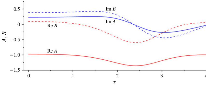
FIGURE 3. Evolution of A and B with \tau ; m = 1/2 , f = 4/3 , \mathcal{N} = 4/3 .
