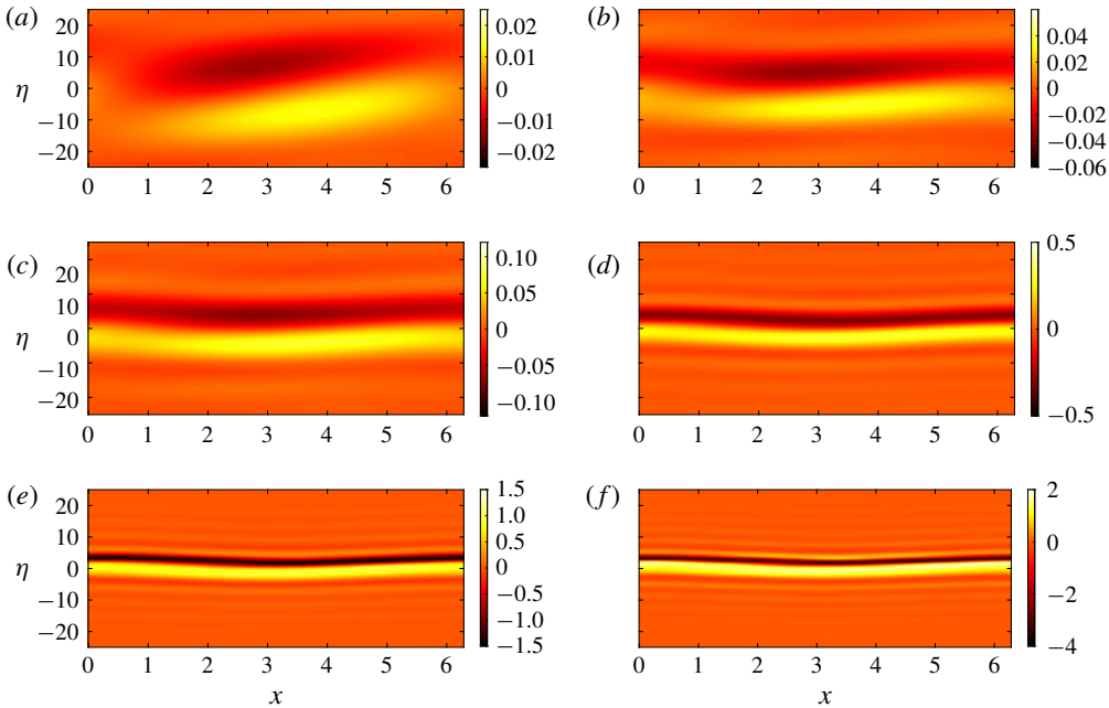
FIGURE 5. Snapshots of vertical vorticity \zeta within the baroclinic critical layer near y = \mathcal{N} = 4/3 , plotted as a colour map on the (x, \eta) -plane for (a) \tau = 0.3 , (b) \tau = 0.45 , (c) \tau = 0.6 , (d) \tau = 1 , (e) \tau = 1.5 and (f) \tau = 1.8 . The domain plotted is |\eta| < 25 , corresponding to |y - \mathcal{N}| < 0.39 , at cross-section z = 0 and over one streamwise wavelength of the forcing pattern. ( \varepsilon_0 = 0.05 , \varepsilon = 0.0062 , m = 1/2 , f = 4/3 , \mathcal{N} = 4/3 .)
