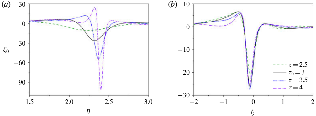
FIGURE 7. (a) Evolution of \zeta_0 near \eta_c = 2.43 at the times indicated. (b) Scaled profiles, \zeta_0 e^{-\sigma_c(\tau-\tau_0)} against \xi = (\eta - \eta_c) e^{\sigma_c(\tau-\tau_0)} , choosing \tau_0 = 3 ; ( m = 1/2, f = 4/3, \mathcal{N} = 4/3 ).
