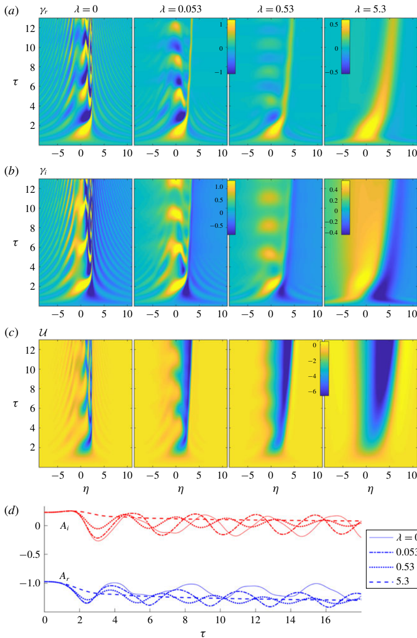
FIGURE 9. Solutions of the modified canonical model, showing (a) \gamma_r , (b) \gamma_i and (c) U , for m = 1/2 , f = 4/3 and \mathcal{N} = 4/3 , c_1 = 0.238 , c_2 = 0.219 with the values of \lambda indicated (and corresponding to the three columns). The colour map is the same in the first three images of (a) and (b), but not the rightmost image. The quasi-steady-wave amplitude A = A_r + iA_i for the four computations is shown in (d).
