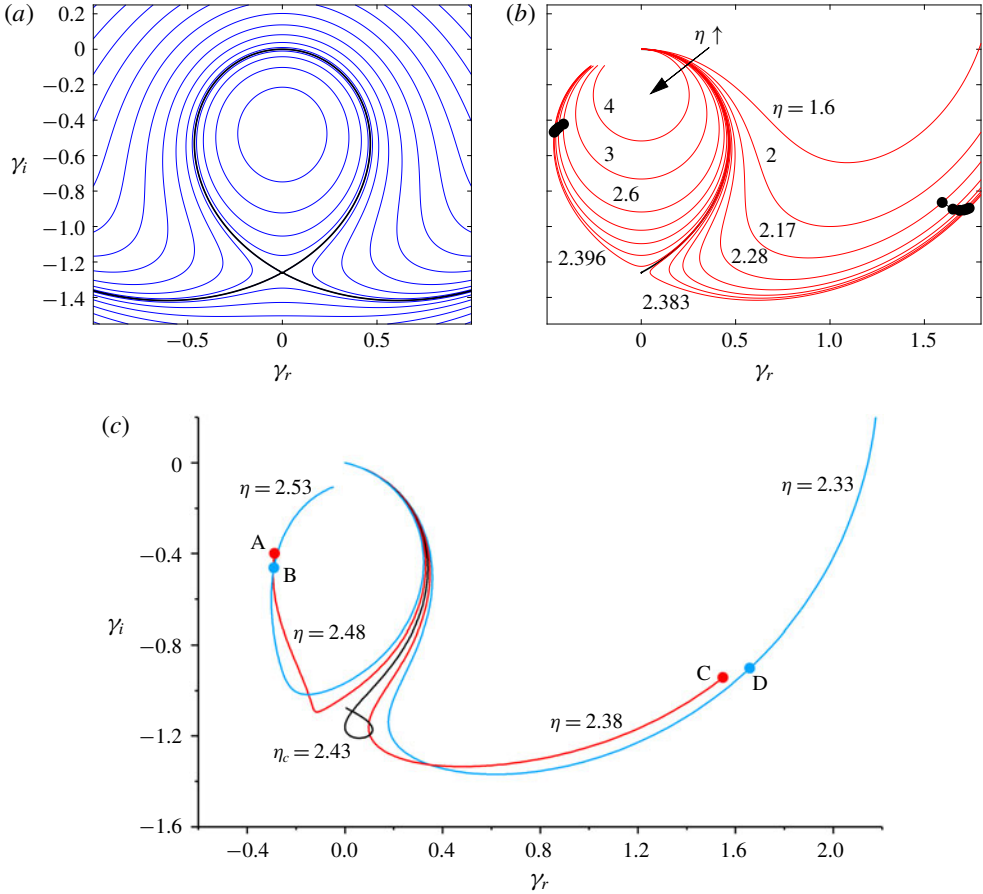
FIGURE 6. Phase portraits of (\gamma_r, \gamma_i) for (a) the Hamiltonian system (5.23) with \eta = 3/\sqrt[3]{2} and various H , with the thicker line indicating H = 0 , (b) trajectories from the point (\gamma_r, \gamma_i) = (0, 0) for a selection of values of \eta and (c) the numerical solution of § 5.3, at the five values of \eta indicated. The black points in (b) and the (red and blue) pairs marked (A,B) and (C,D) in (c) have the same values of |\eta - \eta_c|e^{\sigma\tau} .
