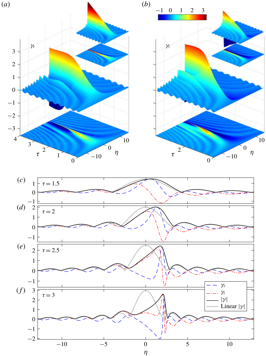
FIGURE 4. (a) Real and (b) imaginary parts of the critical-layer density perturbation \gamma(\eta, \tau) , shown as surfaces above the (\eta, \tau) -plane. To prevent the viewing perspective from obscuring parts of the solution, we also show density maps of the solutions underneath. The insets show corresponding plots of the linear solution in (5.20). Panels (c–f) plot snapshots of \gamma(\eta, \tau) at the times indicated; the linear result for |\gamma(\eta, \tau)| is also included. ( m = 1/2 , f = 4/3 , \mathcal{N} = 4/3 .)
