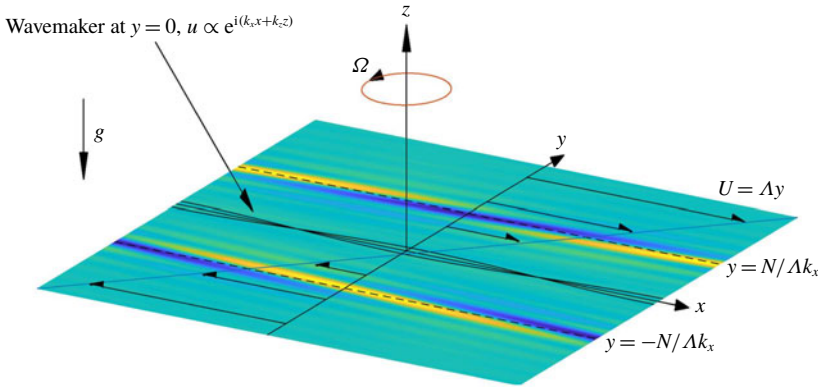
FIGURE 1. Sketch of the model. A wavemaker with wavenumbers k_x and k_z is imposed at y = 0 , and baroclinic critical levels are forced at y = \pm N/(\Delta k_x) , corresponding to dimensionless locations \pm \mathcal{N} , where \mathcal{N} = N\Lambda^{-1} . The shading represents a rendering of the density perturbation based on the linear theory of §3.
