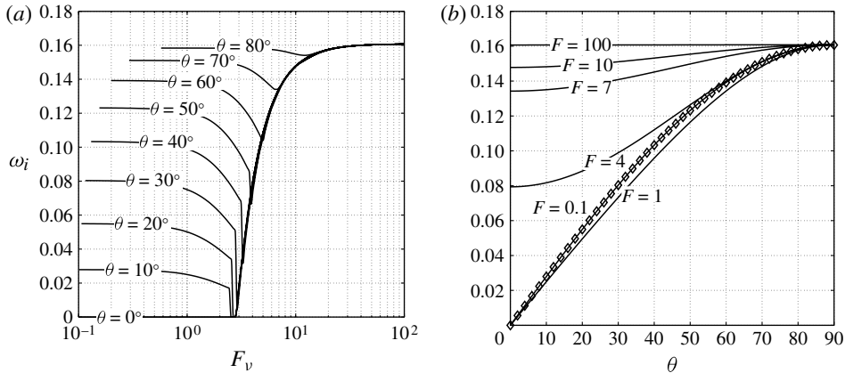
FIGURE 4. Characteristics of the most unstable mode (two-dimensional sinuous KH mode). (a) Growth rate as a function of F_v = F/\cos\theta for fixed inclination angles; (b) growth rate as a function of \theta for fixed Froude numbers. The symbols correspond to variations in \sin\theta as predicted by the small-Froude analysis.
