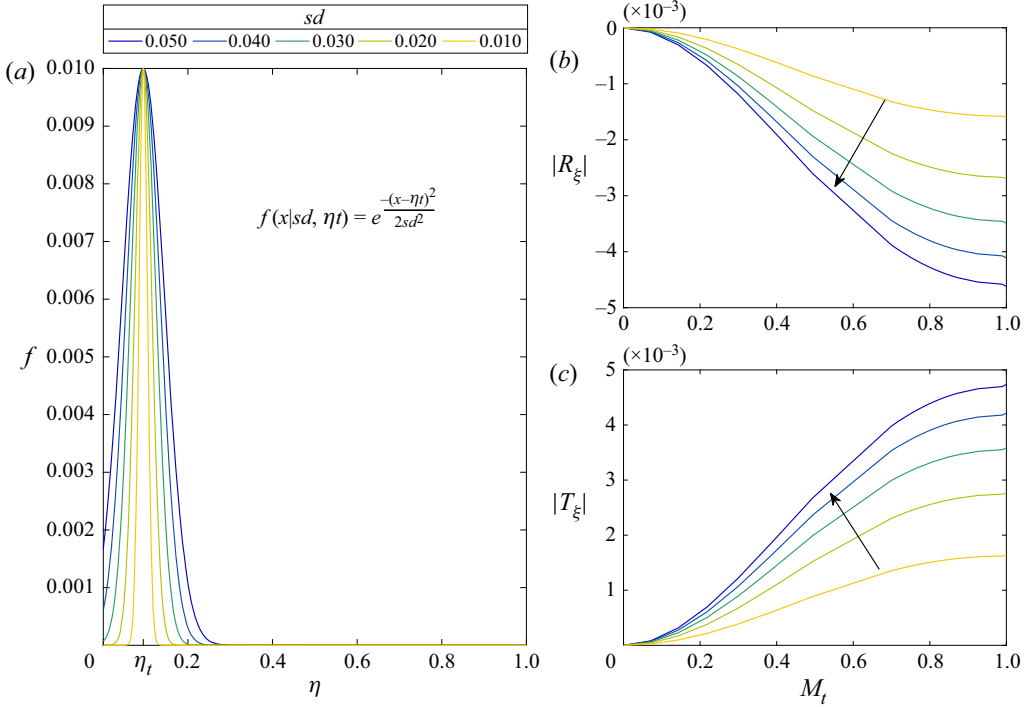
Figure 11. Effect of friction profile. (a) Friction as a function of the spatial distance. (b) Reflection and (c) transmission coefficients as a function of the throat Mach number for different standard deviations, sd .
