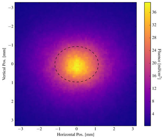
Fig. 3. Beam intensity imaged by an intensified CCD camera. An \text{Al}_2\text{O}_3 scintillator intercepts the beam at the target plane. The dotted line shows the beam profile with 2 mm FWHM.
