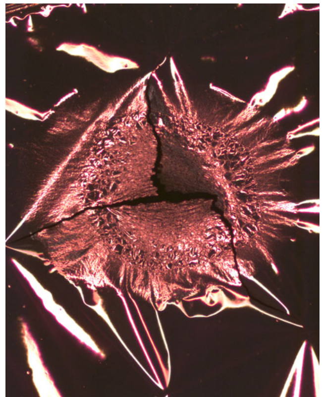
Fig. 5. A microscope image of a 0.3 \mu\text{m} Sn foil after being struck by one helium beam pulse ( 40 \text{ mJ/cm}^2 , 1 MeV) shows surface structures from melting and re-solidification and cracks from rupturing. The field of view is \approx 6 \text{ mm} .
