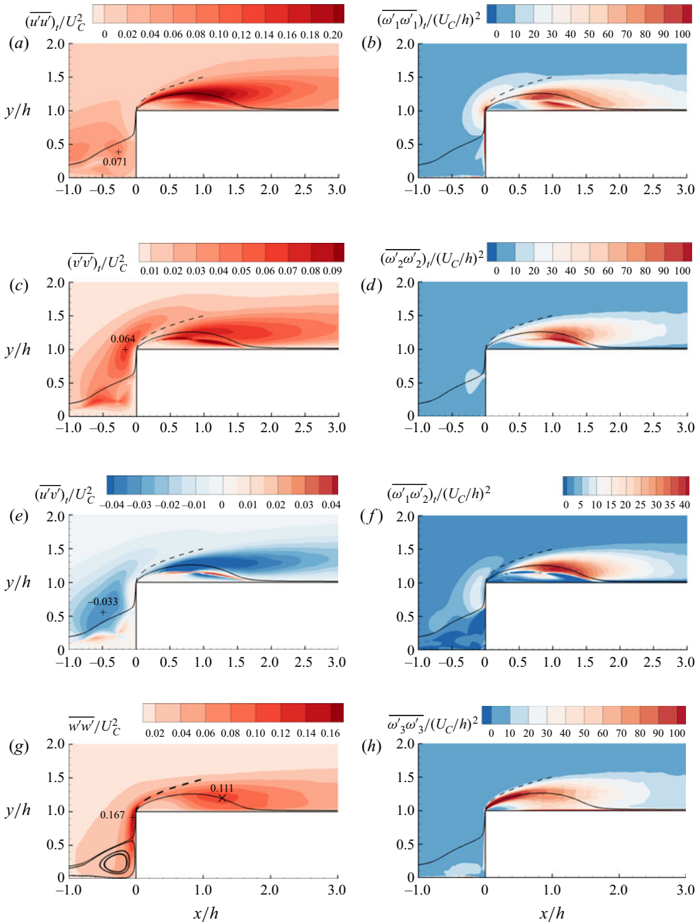
Figure 7. Contours of mean-square values of fluctuating velocity and vorticity along and perpendicular to the mean streamlines superimposed with mean separating streamlines (solid lines): (a) (\overline{u'u'})_t , (b) (\overline{\omega'_1\omega'_1})_t , (c) (\overline{v'v'})_t , (d) (\overline{\omega'_2\omega'_2})_t , (e) (\overline{u'v'})_t , (f) (\overline{\omega'_1\omega'_2})_t , (g) \overline{w'w'} and (h) \overline{\omega'_3\omega'_3} . In (a,c,e,g), symbol + marks the local peak upstream of the step. The dashed line represents the location of the PSL.
