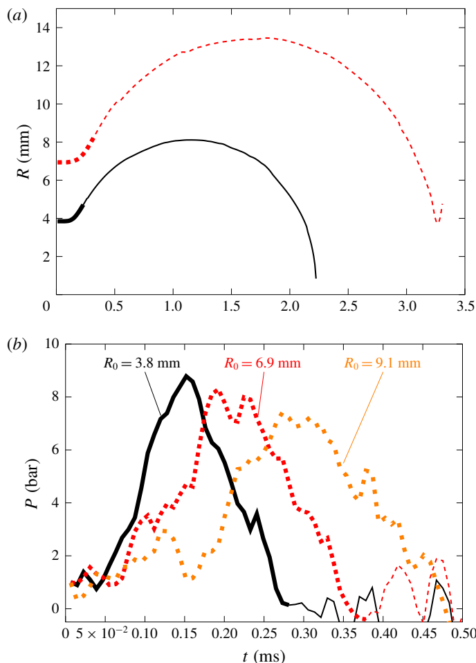
FIGURE 3. (Colour online) Evolution of bubble radius (a) and inner pressure (b), deduced from (3.4), for a gap thickness h = 2.3 mm and initial radius R_0 = 3.8, 6.9 and 9.1 mm (respectively, black continuous line, red dashed line, and orange loosely dashed line). The radius evolution of the largest bubble is not represented as it becomes larger than the camera view field. Note that the overpressure (thick lines) period is short in comparison with the bubble expansion period. Because of the liquid inertia, the bubble continues to expand even after the pressure has vanished (thin lines). The transition between the overpressure period and the depressurization period is set arbitrarily.
